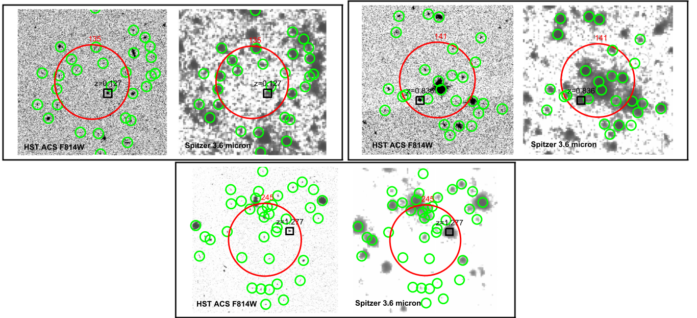
Figure 16. Postage-stamp images of the 30'' \times 30'' sky around NuSTAR sources ID 135, 141, and 245 (from top to bottom). For each source the HST ACS F814W and Spitzer IRAC ( 3.6 \mu\text{m} ) images are presented. Red circles = NuSTAR position; green circles = optical catalog sources; black squares = sources with spectroscopic identification.
