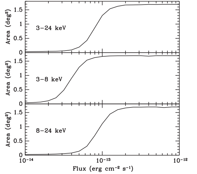
Figure 7. Sky coverage at 99% reliability DET_ML level. Top: 3–24 keV band; middle: 3–8 keV band; bottom: 8–24 keV band.
