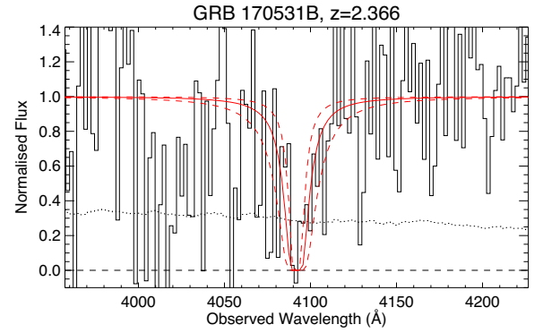
Figure A33. Fit of the red wing of \text{Ly}\alpha for the GRB 170531B GTC/OSIRIS spectrum.
