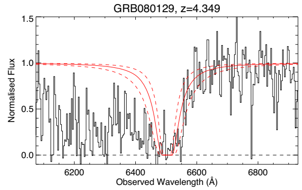
Figure A3. Fit of the red wing of \text{Ly } \alpha for the GRB 080129 VLT/FORS1 spectrum.
