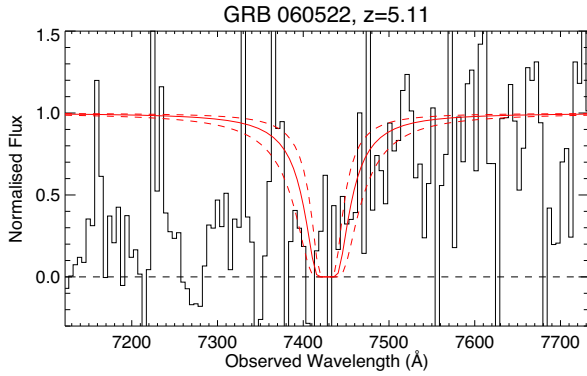
Figure A1. Fit of the red wing of \text{Ly } \alpha for the GRB 060522 Keck-I/LRIS spectrum.
