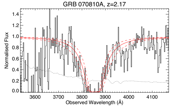
Figure A2. Fit of the red wing of \text{Ly } \alpha for the GRB 070810A Keck-I/LRIS spectrum.
