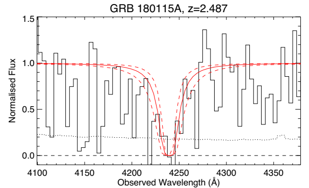
Figure A34. Fit of the red wing of \text{Ly}\alpha for the GRB 180115A GTC/OSIRIS spectrum.
