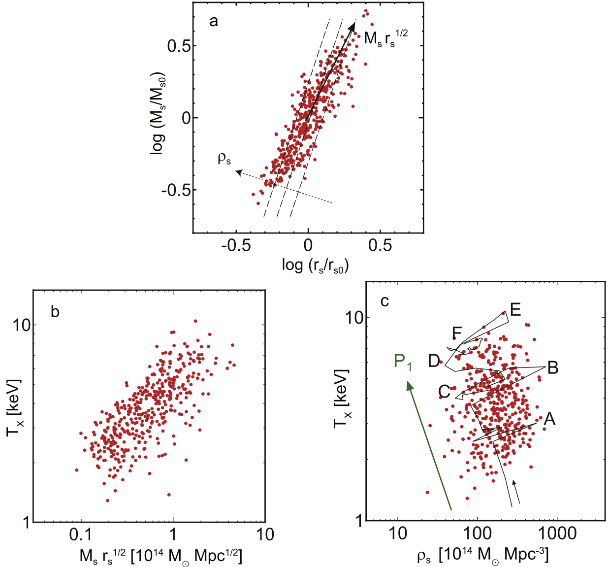
Figure 5. (a) Projection of the MUSIC data points in Figure 3(a) on the \log r_s – \log M_s plane. The normalizations of the axes are the same as those in Figure 3. Each dashed line satisfies \rho_s = \text{const} and the value of the constant increases in the direction of the thin dotted arrow. The thick solid arrow represents a line r_s \propto M_s^{1/2} , and the value M_s r_s^{1/2} increases in the direction. (b) T_X is plotted against M_s r_s^{1/2} . (c) T_X is plotted against \rho_s . Evolution of a typical cluster belonging to FB0+FB1 is shown in the solid line. Prominent features are marked by the labels A, B, ..., F. The cluster and the labels are the same as those in Figure 6. The green arrow shows the projected direction of P_1 for the MUSIC data.
