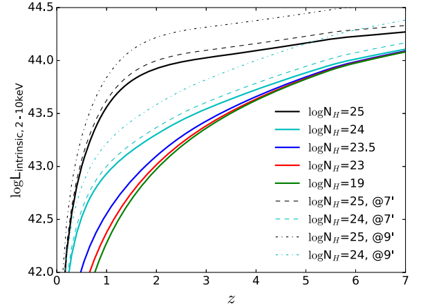
Figure 25. Boundary of detectable regions in L_X - z space with respect to different N_H . Solid lines correspond to the aimpoint region (off-axis angle < 1.5' ). Dashed lines and dash-dotted lines correspond to off-axis angles of 7' and 9' , respectively.
