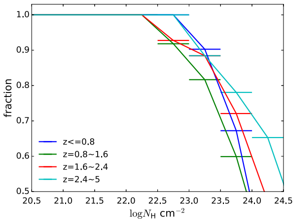
Figure 29. Fraction of sources detectable within our sample with a given N_H , computed for the luminosity range \log L within 42–45, in four redshift bins.
