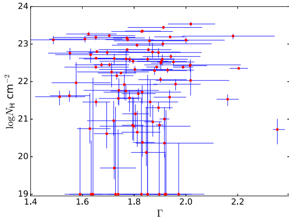
Figure 13. Scatter plot of the best-fit \Gamma and N_H . Only the sources with free \Gamma are shown here. Error bars correspond to 1\sigma .
