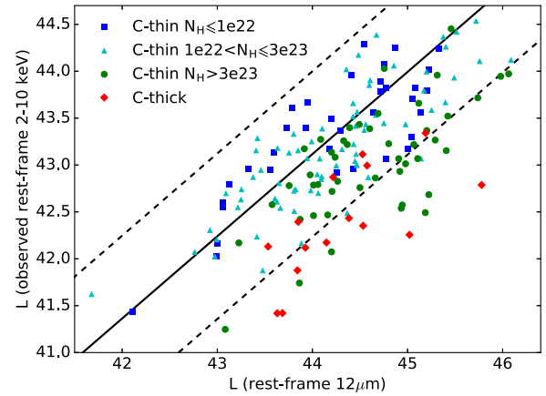
Figure 7. Scatter plot of the rest-frame 2–10 keV observed X-ray luminosity and the total rest-frame 12\mu\text{m} luminosity. The sources are divided into four subsamples according to the N_H . The solid line corresponds to the best-fit L_{2-10 \text{ keV, intrinsic}} - \log L_{12\mu\text{m}} correlation, and the dashed lines represent its 2\sigma scatter.
