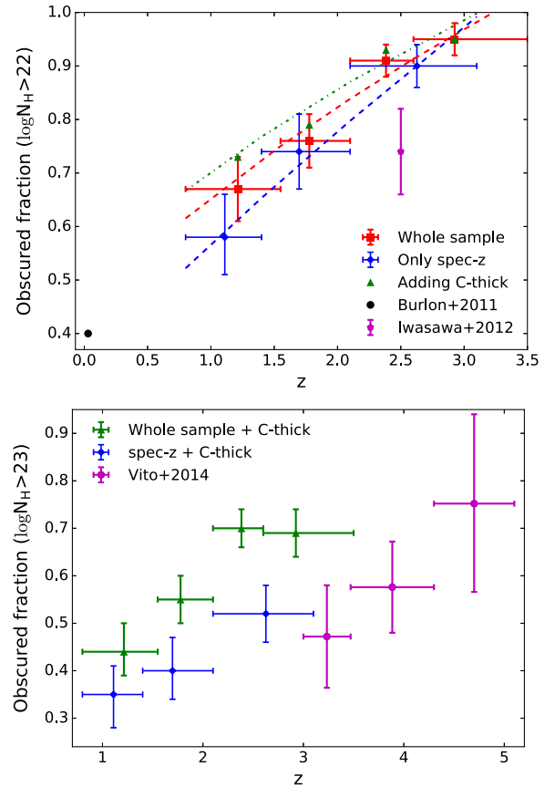
Figure 32. Upper panel: fractions of sources with \log N_H > 22 in the four bins ( 0.8 < z < 3.5, 43.5 < \log L < 44.2 ) as shown in Figure 31 and best-fit lines. Results obtained from the whole “completeness” = 24 sample are plotted in red, the spectroscopic-z subsample in blue. Results obtained after adding the Compton-thick sources to the whole sample are shown in green; the error bars are omitted for simplicity. The Burlon et al. (2011) and Iwasawa et al. (2012) results correspond to \log L \approx 43.85 and \log L \approx 44.2 , respectively. Lower panel: fractions of sources with \log N_H > 23 . Results from our sample adding the Compton-thick sources are plotted in green, from the spectroscopic-z subsample adding the Compton-thick sources are plotted in blue. Results from the 42.85 < \log L < 44.5 sample of Vito et al. (2014) are plotted in magenta.
