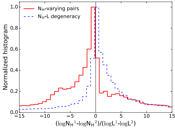
Figure 11. Resampled k distributions, calculated between each pair of N_H variable spectra (red) and each pair of random values of the same spectrum (blue). The histograms are normalized to the peak value.
