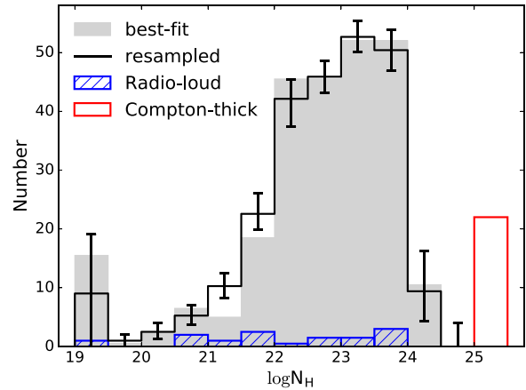
Figure 12. Observed N_H distribution. The gray filled histogram shows the best-fit N_H distribution of the Compton-thin sources. All the sources with best-fit \log N_H \leq 19 are plotted in the leftmost bin. Compton-thick sources are shown in the red histogram at \log N_H > 25 . The black empty histogram shows the resampled N_H distribution of the Compton-thin sources, using mock values generated according to the statistical error on N_H . The 1\sigma error bars of the histogram are obtained from the scatter of 1000 resampled histograms. The blue dashed histogram corresponds to the 13 radio-loud sources.
