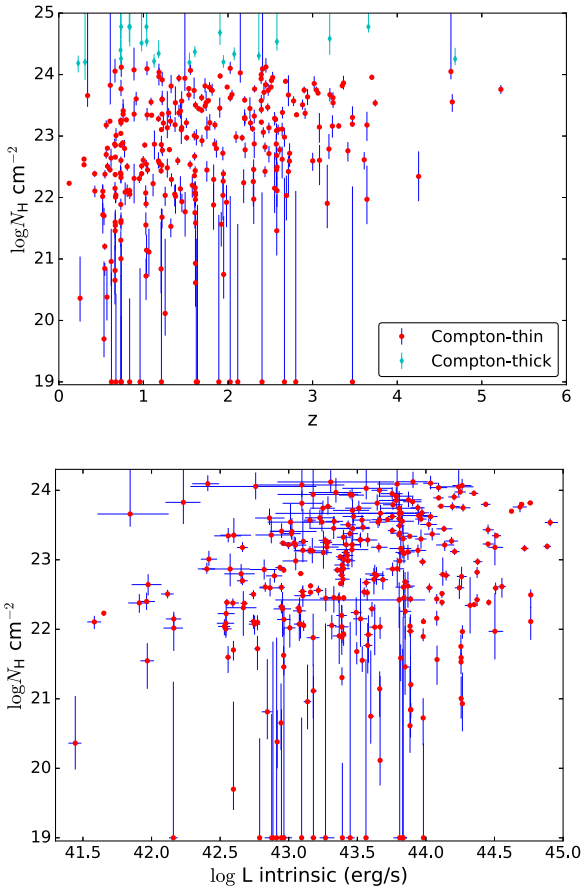
Figure 15. Best-fit N_H vs. redshift. Error bars correspond to 1\sigma . Some sources with very low or very high N_H have very large uncertainties. Scatter plot of the best-fit N_H and rest-frame 2–10 keV unabsorbed luminosities of the Compton-thin sources. Error bars correspond to 1\sigma .
