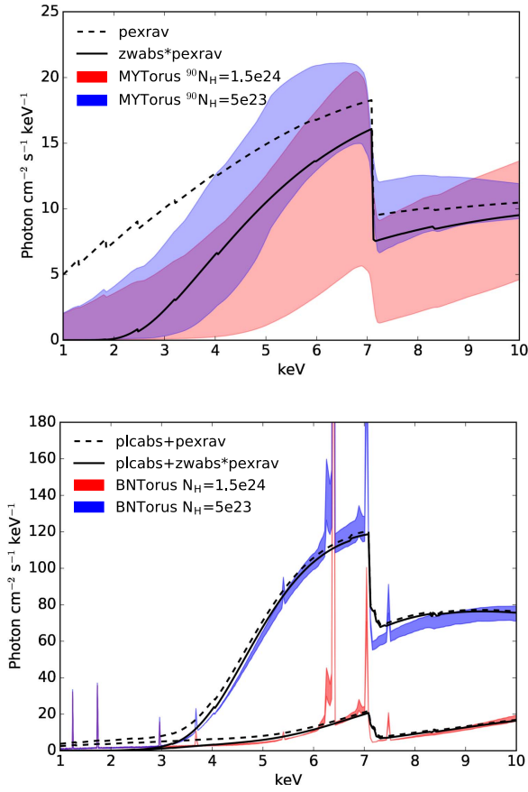
Figure 6. Upper panel: the reflection model adopted in this work ( \text{zwabs} \times \text{pexrav} with an N_{\text{H}} of 10^{23} \text{ cm}^{-2} , black solid line) compared with MYTorus reflection models (color filled regions) with diameter column densities of {}^{90}N_{\text{H}} = 5 \times 10^{23} \text{ cm}^{-2} (blue) and {}^{90}N_{\text{H}} = 1.5 \times 10^{24} \text{ cm}^{-2} (red) between inclination angles of \theta = 0^\circ (face-on) and \theta = 90^\circ (edge-on). The unabsorbed \text{pexrav} model is plotted with a dashed black line. All the models are derived from the same intrinsic primary power-law and have z = 0 . Lower panel: the model of transmitted power-law plus reflection adopted in this work ( \text{plcabs} + \text{zwabs} \times \text{pexrav} , black solid lines) compared with BNTorus models (color filled regions) in two cases with N_{\text{H}} = 5 \times 10^{23} \text{ cm}^{-2} (blue) and N_{\text{H}} = 1.5 \times 10^{24} \text{ cm}^{-2} (red), respectively. The filled ranges correspond to torus opening angles between \theta_{\text{torus}} = 30^\circ and \theta_{\text{torus}} = 60^\circ . Without the self-absorption, the \text{plcabs} + \text{pexrav} model is plotted with the black dashed line. All the models have z = 0 . They are all derived from the same intrinsic primary power-law, but the normalizations of the \text{plcabs} -based models are multiplied by factors of 75% and 50% in the cases of N_{\text{H}} = 5 \times 10^{23} \text{ cm}^{-2} and N_{\text{H}} = 1.5 \times 10^{24} \text{ cm}^{-2} , respectively.
