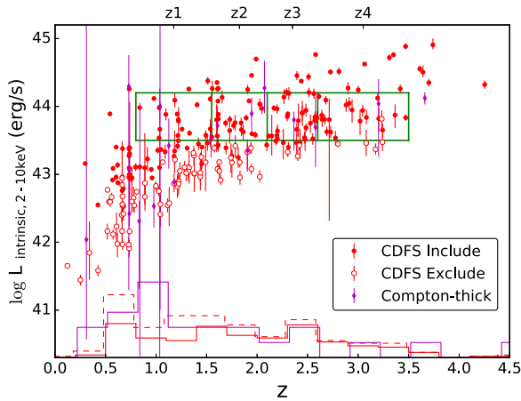
Figure 31. Scatter plot of the AGN sample in the luminosity—redshift space, with 90% errors on luminosity. The \log N_H < 24 N_H -complete subsample is plotted with red solid points (marked as “Include”) and the other Compton-thin sources with red empty points (marked as “Exclude”). At the bottom, the normalized redshift distributions of the complete subsample (“Include”) and the whole sample (“Include”+“Exclude”) are shown as red solid and dashed histograms, respectively. The Compton-thick sources are also shown with the magenta points and the blue histogram. The four green boxes, which are marked as z1 , z2 , z3 , and z4 , are the regions selected to analyze the N_H dependence on redshift. Empty points are excluded from this analysis even if they fall in the selected bins.
