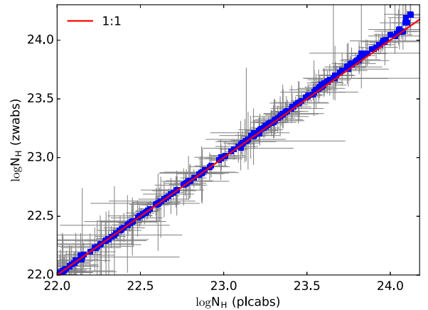
Figure 17. N_H measured using zwabs and plcab s with 1\sigma error for the Compton-thin sources, whose N_H are well constrained.
