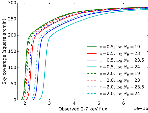
Figure 23. Sky coverage as a function of the 2–7 keV observed flux ( \text{erg cm}^{-2} \text{s}^{-1} ) corresponding to 80 hard-band net counts for a set of N_H values at redshifts of 0.5 (solid lines) and 2 (dashed lines).
