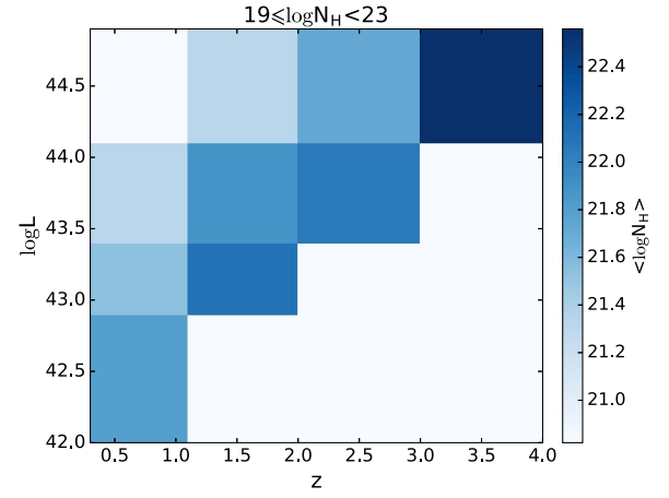
Figure 34. Mean \log N_H in grid, combining CDF-S and C-COSMOS data. Only values below 23 are considered. Values below 19 are taken as 19. White cells are excluded.
