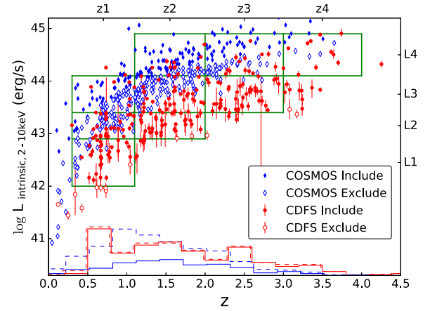
Figure 33. Same as Figure 31, but including C-COSMOS data (red for CDFS-S, blue for C-COSMOS). The selected subsamples are complete for \log N_H < 23 .
