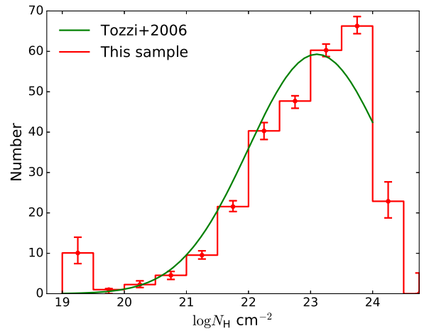
Figure 30. Intrinsic N_H distribution of our whole sample, measured by summing up the intrinsic N_H distributions in the four redshift bins ( z < 5 ) as shown in Figure 27. The 90% percentile luminosity range of our sample is 42.41 \sim 44.45. The green line that is derived from the 1Ms CDF-S by Tozzi et al. (2006), is a log-normal distribution centered at \log N_H = 23.1 with a \sigma = 1.1 and normalized to the number of AGN used in this work between \log N_H of 19 and 24.
