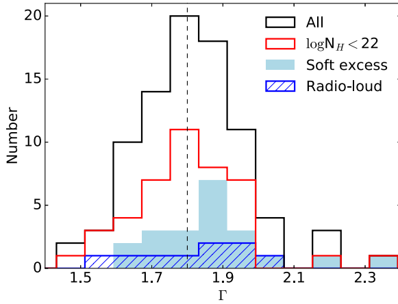
Figure 8. Distribution of best-fit \Gamma for the 95 sources whose \Gamma are well constrained. The vertical line shows the median value of this distribution ( \Gamma = 1.8 ). The red histogram shows the subsample with N_H < 10^{22} \text{ cm}^{-2} . The light-blue filled part corresponds to the sources with a detected soft-excess component. The blue dashed part shows the 9 radio-loud sources.
