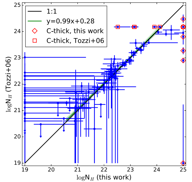
Figure 20. Column densities N_H with 1\sigma errors measured in Tozzi et al. (2006) and in this work in Period I for the sources with consistent redshifts. Sources identified as Compton-thick in Tozzi et al. (2006) and in this work are marked with red squares and red diamonds. We set the \log N_H of our Compton-thick sources at 25. The linear fitting result and 1\sigma confidence interval are plotted with green line and shade.
