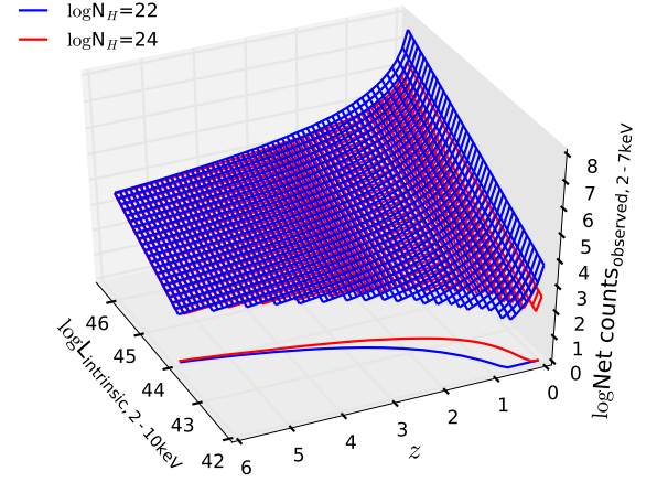
Figure 24. Conversion surfaces from any point in the L_X - z space to hard-band observed net counts, obtained at the aimpoint with a \log N_H of 22 (blue grid and line) and 24 (red grid and line). Only the parts above 80 net counts of the surfaces are shown. The lines in the L_X - z space at the base are projections of the intersections of the two surfaces with the plane where the net counts = 80.
