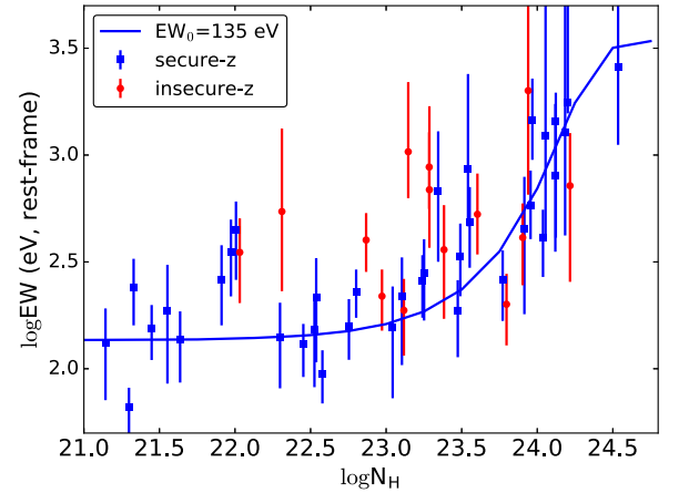
Figure 10. Scatter plot of \log N_H and \log EW of the detected narrow Fe K \alpha line. Sources with secure and insecure redshift measurements are plotted in blue and red, respectively. The blue line shows our model of the line with an N_H -independent flux and EW = 135 eV when unobscured.
