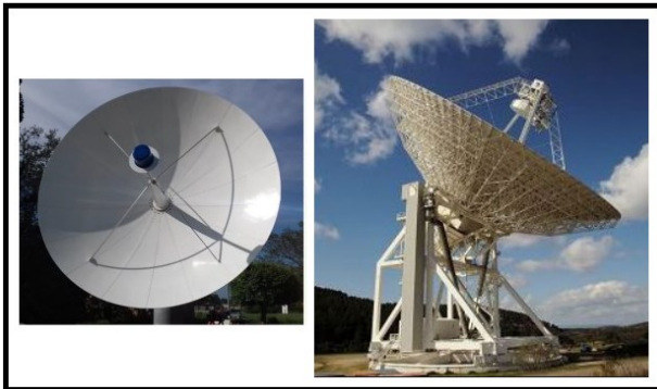
Fig. 1. The P-band BIRALET system. In particular, on left the TRF, on right the SRT.
