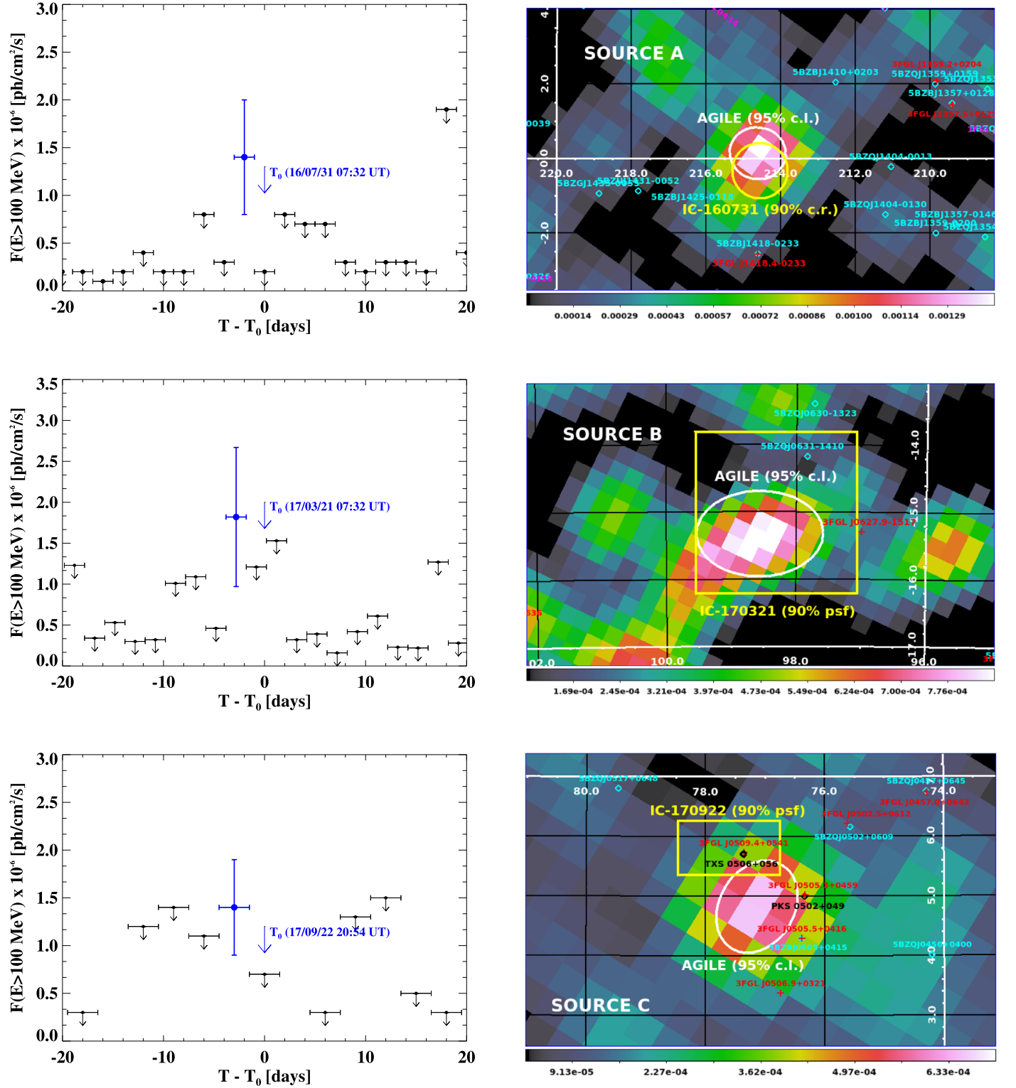
Figure 1. Results of the AGILE-GRID standard analysis for the three Sources A (upper panel), B (middle panel) and C (lower panel) of Table 1. Left panels: gamma-ray lightcurves above 100 MeV around the IceCube T_0 . Right panels: maps in equatorial coordinates (J2000) of gamma-ray intensity above 100 MeV in ( \text{ph cm}^{-2} \text{ s}^{-1} \text{ sr}^{-1} ) corresponding to the gamma-ray detection before T_0 shown on the left. The AGILE 95% confidence level (c.l.) location contours are shown in white; the IceCube error boxes or circles are shown in yellow. A systematic error of 0.1 should be added to each AGILE source determination. The positions of the classified AGNs from the BZCAT Catalog (Massaro et al. 2015) and the FERMI-LAT 3FGL gamma-ray sources (Acero et al. 2015) are shown in cyan and red, respectively.
