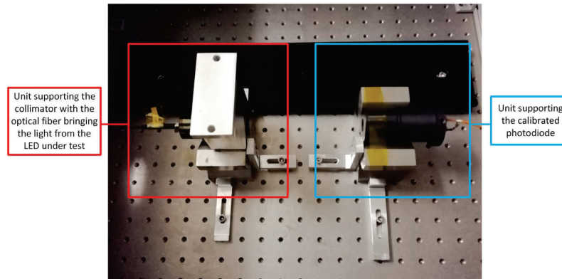
Figure 8. Setup for the calibration of the LEDs.
