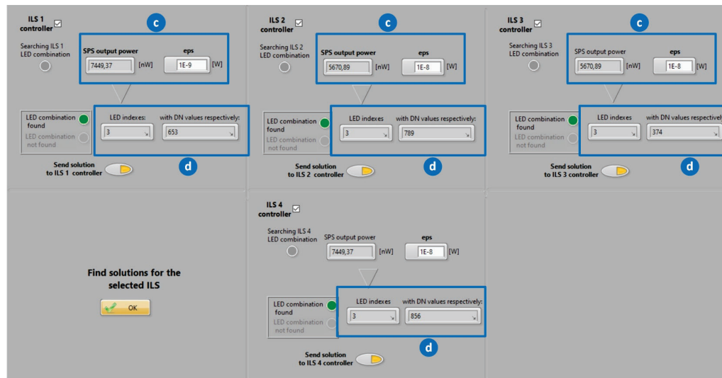
Figure 6. GUI of the module that calculates the best combination of the LED DAC levels to obtain the expected output power.
