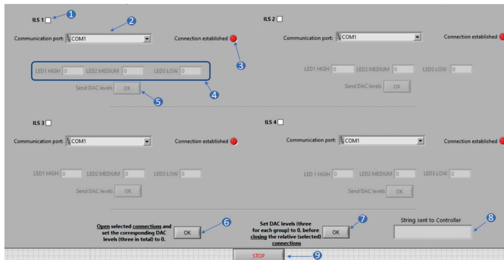
Figure 7. GUI to command the ILS LEDs.
