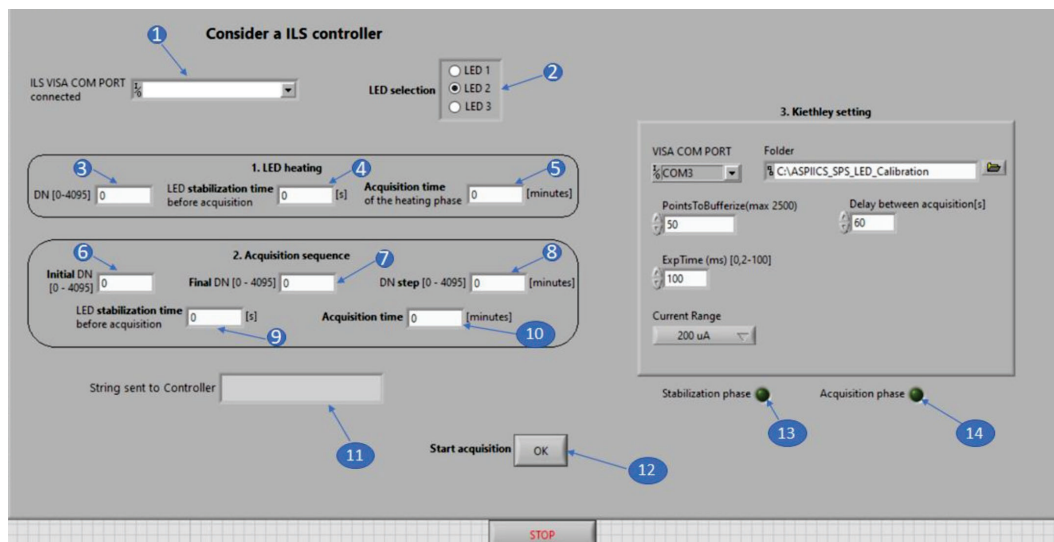
Figure 9. GUI to perform dynamic setting of the the ILS LEDs.
