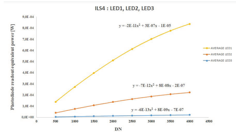
Figure 10. Typical calibration curve of the LED sources.
