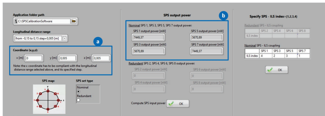
Figure 5. GUI of the module to estimate the input power on the SPS for an user-set formation alignment configuration.
