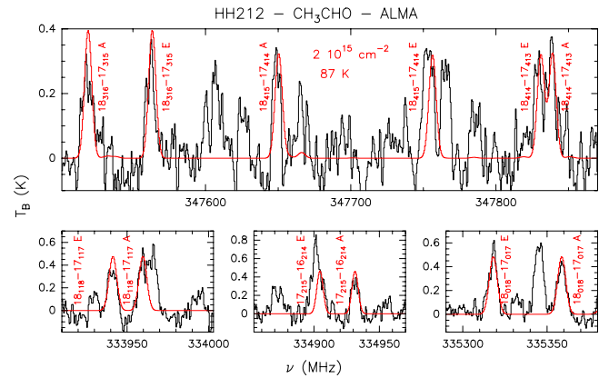
Fig. 2. CH 3 CHO emission (in T_B scale) extracted at the MM1 position. The four panels show the frequency intervals where the CH 3 CHO lines are located (see Table 1 for those unblended with other lines). The red line shows the synthetic spectrum which best reproduces the observations assuming LTE and optically thin emission obtained with the GILDAS–Weeds package (Maret et al. 2011) with source size = 0''.3 , T_{\text{rot}} = 87 \text{ K} , N_{\text{CH}_3\text{CHO}} = 2 \times 10^{15} \text{ cm}^{-2} , FWHM linewidth = 5.0 \text{ km s}^{-1} , and LSR velocity = +1.7 \text{ km s}^{-1} (see footnote 2).
