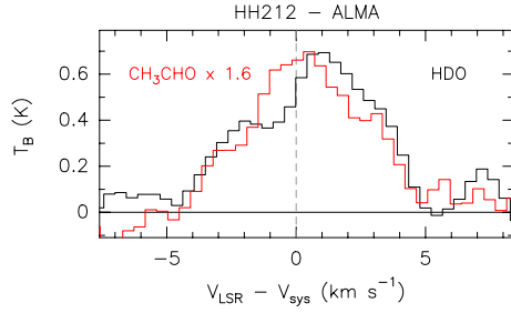
Fig. 3. Comparison between HDO( 3_{3,1}-4_{2,2} ) (black line) and CH 3 CHO( 18_{0,18}-17_{0,17} )A (red, multiplied by a factor of 1.6) as observed towards HH212-MM1 (in T_B , scale). The vertical dashed line defines the velocity with respect to V_{\text{sys}} = +1.7 \text{ km s}^{-1} (see footnote 2).
