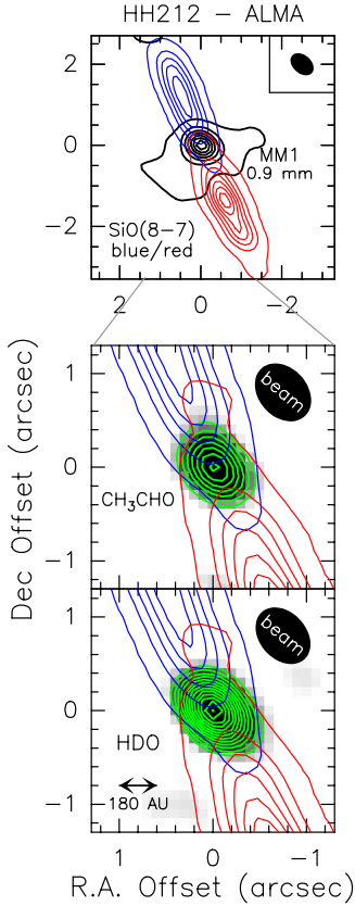
Fig. 1. Upper panel: the HH212 protostellar system as observed by ALMA–Band 7 (Codella et al. 2014). Blue/red contours plot the blue-/redshifted SiO(8–7) jet at \pm 8 \text{ km s}^{-1} from V_{\text{sys}} , overlaid on the 0.9 mm continuum (black contours). Positions are with respect to the coordinates reported in Sect. 2. The filled ellipse shows the synthesised beam (HPBW) for SiO: 0''.63 \times 0''.46 (PA = 49^\circ ). Middle panel: zoom-in of the central region: the CH 3 CHO( 18_{0,18}-17_{0,17} )A emission integrated over \pm 5 \text{ km s}^{-1} (green contours and grey scale) overlaid on the SiO jet. First contours and steps are 5\sigma (50 mJy beam ^{-1} \text{ km s}^{-1} ) and 2\sigma , respectively. The HPBW is 0''.69 \times 0''.52 (PA = 42^\circ ). Bottom panel: same as middle panel for HDO. The HPBW is 0''.68 \times 0''.51 (PA = 42^\circ ).
