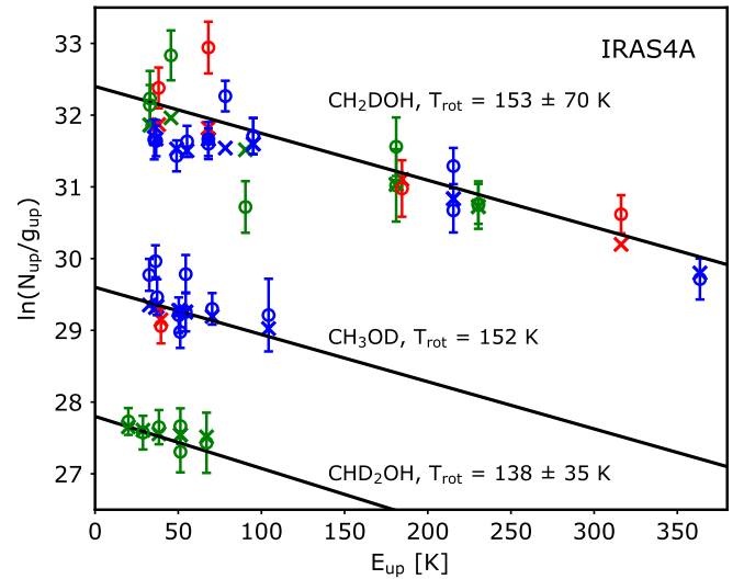
Fig. 5. Rotational and population diagrams of deuterated methanol isotopologues ( \text{CH}_2\text{DOH} , \text{CH}_3\text{OD} , and \text{CHD}_2\text{OH} ) derived towards NGC1333-IRAS4A for source sizes derived from the PD analysis of the methanol population distribution ( 0''.20 ; see Taquet et al. 2015). Red, green, and blue symbols represent transitions at 145, 165, and 225 GHz, respectively. The \text{CH}_3\text{OD} and \text{CHD}_2\text{OH} levels have been artificially shifted by -1.5 and -4 for sake of clarity. Observational data are depicted by the diamonds. Crosses show the best fit of the PD to the data. Blue and green symbols represent transitions at 2 and 1.3 mm, respectively. Error bars are derived assuming a calibration uncertainty of 20 % on top of the statistical error. Black straight lines represent the best fit of the rotational diagram analysis, assuming optically thin emission, to the data.
