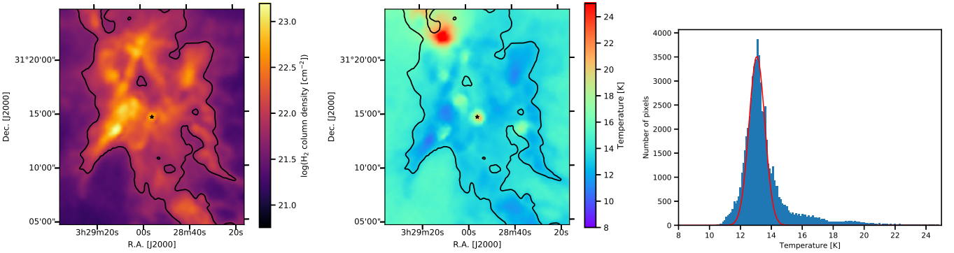
Fig. B.1. H 2 column density (left), dust temperature (center) maps, and dust temperature histogram of the map pixels with A_V > 3 mag (right) of the NGC1333 star-forming region surrounding IRAS2A as observed with the Herschel Space Observatory by the Gould Belt survey (André et al. 2010). The black contour in the maps depicts the 3 mag level. The red curve on the histogram depicts the gaussian fit of the histogram around the histogram peak.
