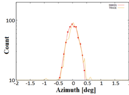
Figure 4. Azimuth analyzer response obtained with 2 different codes, Simion (red) and Trace (yellow).
