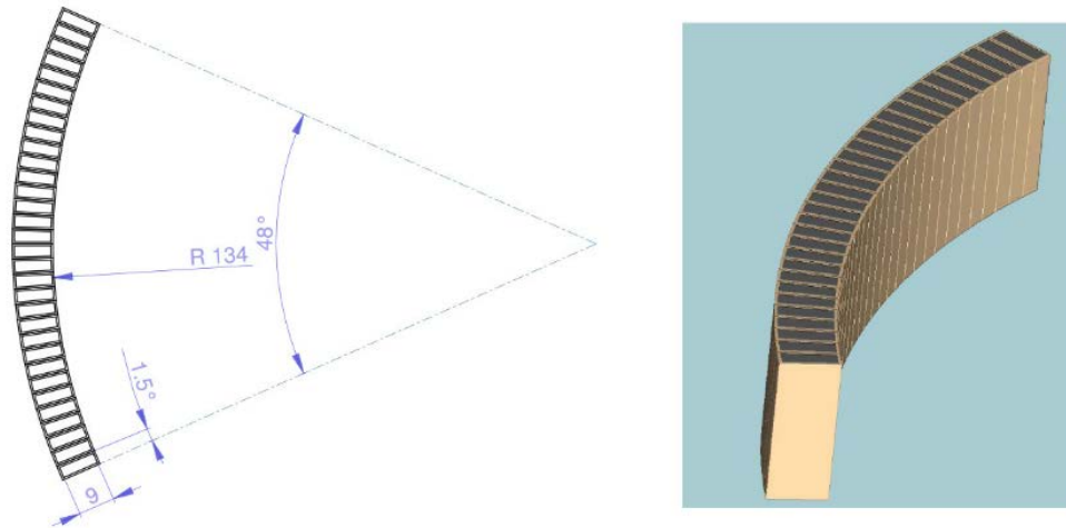
Figure 2. Basic geometry of the CEM detector array that will be used for CSW on THOR. (a) Basic dimensions of the array, and (b) its 3D rendering.
