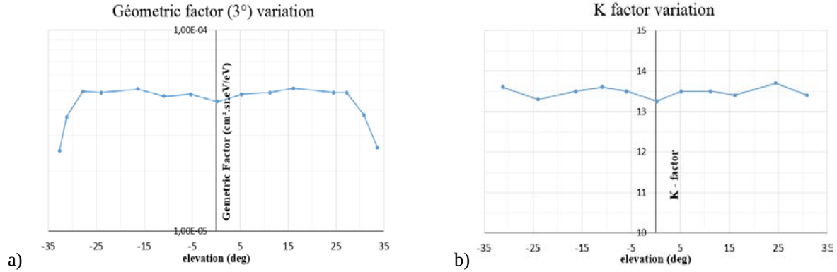
Figure 9. GF (a) and K-factor (b) variation as a function of the elevation angle.
