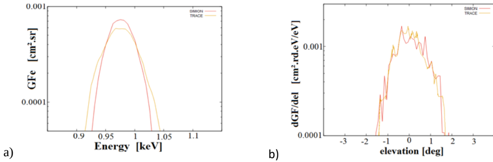
Figure 3. Energy (a) and elevation (b) response obtained with 2 different codes, Simion (red) and Trace (yellow).
