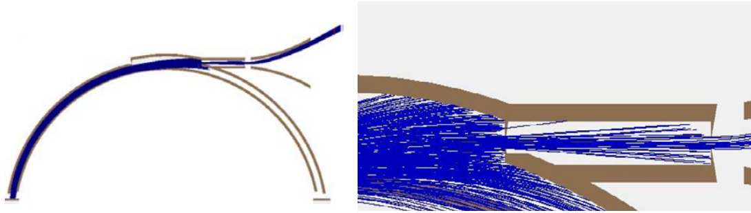
Figure 5. (a) Actual design with sample particle tracing (particles are launched from the detectors on the bottom-left-hand side), and (b) zoom-in on the collimator area to highlight its importance in determining the elevation of accepted particles, and in turn elevation and energy resolutions.
