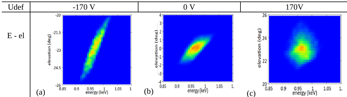
Figure 6. Response function calculated with SIMION showing the transmission rate over the energy and elevation response for three deflector potentials considered: (a) U_{def} = -170 V, (b) 0 V and (c) 170 V. For this simulation both deflectors are polarized in an anti-symmetrical fashion.
