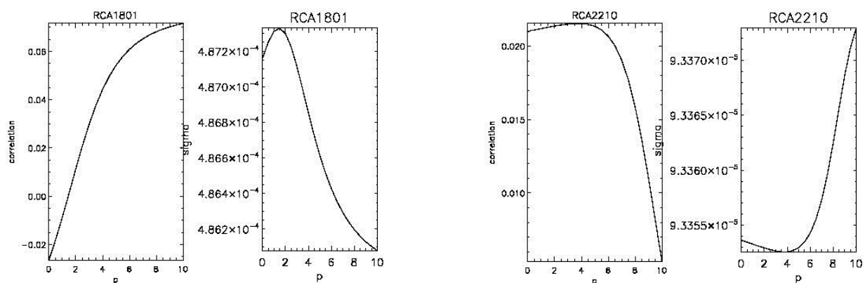
Figure 7 For each channel (LFI 1801 , first and second; LFI 2210, third and fourth panels) they are represented: DIFF DATA – Id HK Correlation with varying p-weight (first and third panels); Sigma Diff with varying p-weight (second and fourth panels). P assumes 21 values from 0 to 1 in steps of 0.05 ( the x axis scale must be multiplied times 0.1). Plots show that the p-value optimizing correlation is the same providing the best sigma after correction.
