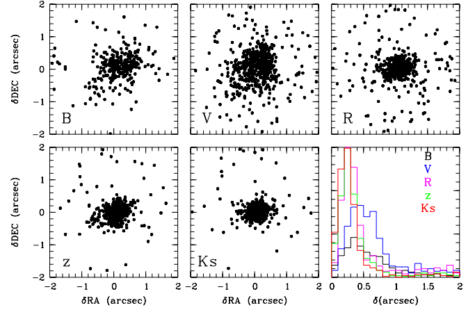
Fig. 1. Astrometric shifts ( \alpha , \delta ) for CL J0152.7-1357 between the objects detected in the i' band and the B , V , R , z' , and Ks bands. The figure at the lower right shows the histograms of the shifts between the i' band and the other bands.
