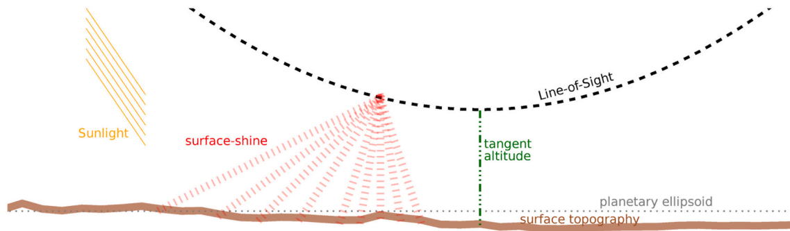
Fig. 8. Sketch of the geometrical configuration of the surface-shine toward a single point along a limb viewing line-of-sight in a plane parallel configuration.
