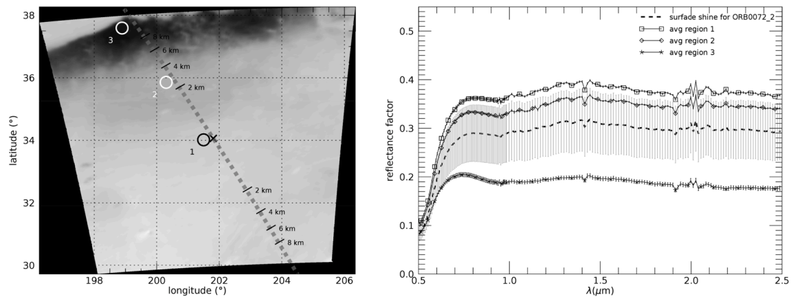
Fig. 9. Example of albedo variability of the terrains underneath a limb line-of-sight. Left panel: The surface track of a given limb observation (actually pertaining to cube ORB0072_2) is drawn as a dashed line over a surface albedo map taken from another nadir-looking OMEGA cube (ORB0351_4 reflectance factor at 1.85 \mu\text{m} , corrected for atmosphere with the method of Langevin et al., 2005). The central cross represents the tangent point (the lowest point of the line-of-sight), whereas the labelled ticks at both sides indicate how the altitude of the line-of-sight changes while going away from the tangent point. Right panel: The three curves with symbols represent surface spectra from different regions close to the line-of-sight (numbered circles in the left hand-side map). The dashed curve with error bars represents the weighted average surface spectrum, described in the text as surface-shine.
