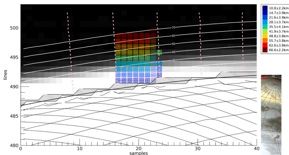
Fig. 2. Illustration of a limb scan mapping from a portion of an OMEGA cube. Surface coordinates grid (thin black lines), planetary limb position (thick black curve), tangent altitude isolines (white curves, labelled in km) and directions of vertical atmospheric columns (dashed lines) are overlapped to the 1.1 \mu\text{m} OMEGA-SWIR reflectance image (grey-scale). Individual pixels assigned to a given limb scan are filled with colors associated with the tangent altitude bins detailed in the legend. The line-filled region encompasses those OMEGA pixels, excluded from the scan, whose footprint is likely crossing the limb. The bottom-right panel shows a larger view of the cube where the limb position is highlighted by the red rectangle. (For interpretation of the references to colour in this figure legend, the reader is referred to the web version of this article.)
