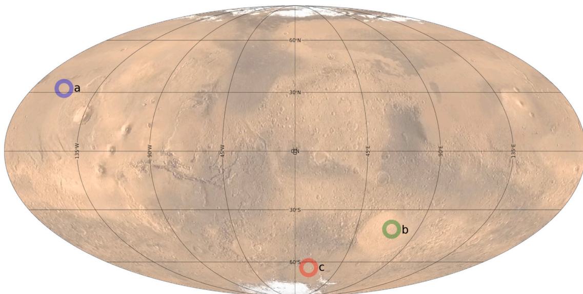
Fig. 1. Location of the limb tangent regions for the selected OMEGA limb scans listed in Table 1.
