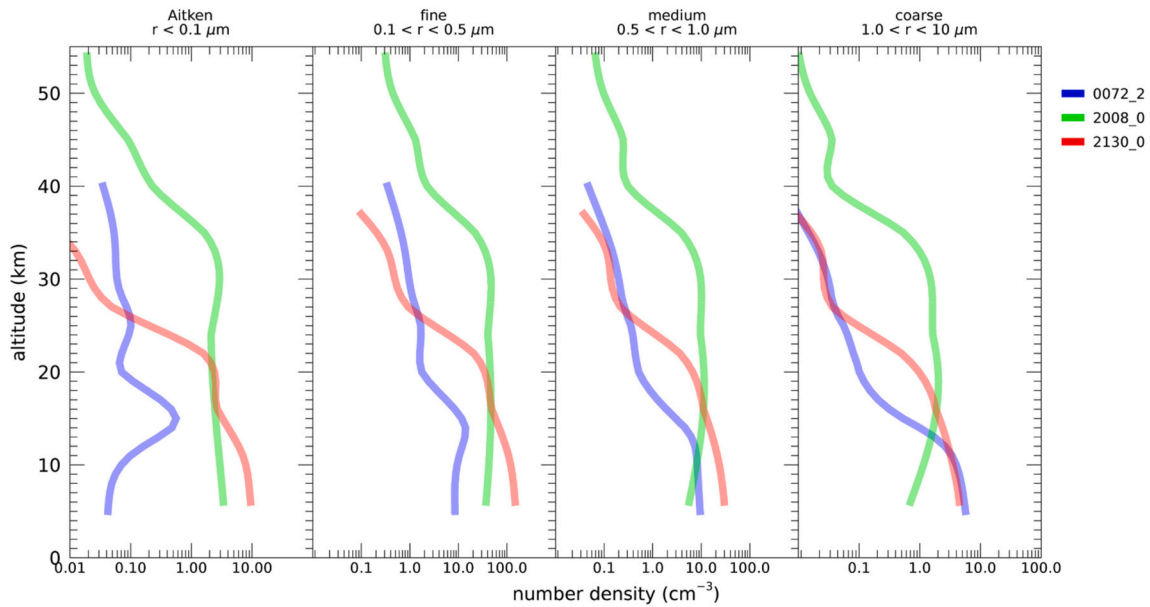
Fig. 14. Vertical profiles of retrieved dust number density for four size classes of grains. Nanometer particles (Aitken mode) are shown in the left panel. Sub-micrometer fine and medium ones are in the middle panels, while coarser micrometer particles are shown in the right panel.
