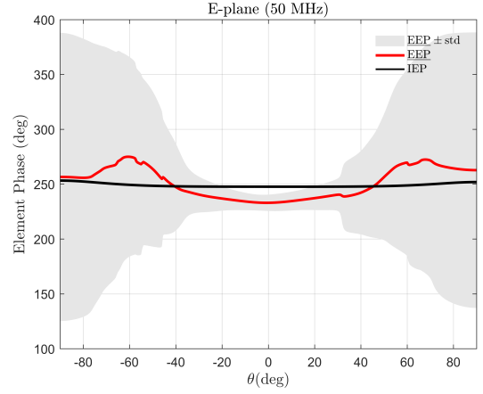
Fig. 11. Average embedded element pattern (EEP) phase, compared to isolated element pattern, 50 MHz, also showing 1\sigma envelope.
