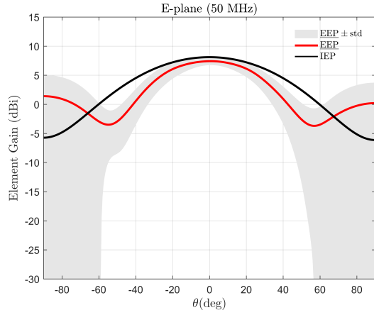
Fig. 8. Average embedded element pattern gain (EEP), compared to isolated element pattern, 50 MHz, also showing 1\sigma envelope.
