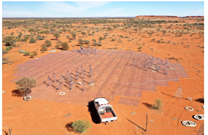
Fig. 3. A "drone's eye" view of the AAVS1.5 array under construction, May 2019. Credits: ICRAR/Curtin.
