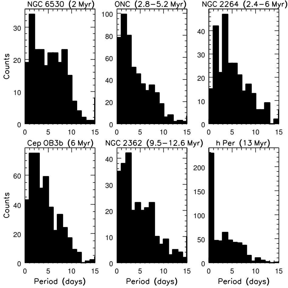
Fig. 16. Comparison of the period distributions obtained for various young clusters of different ages, in the mass range 0.1\text{--}2\,M_{\odot} . The clusters are, from left to right , from top to bottom : NGC 6530 (age of \sim 2 Myr, Bell et al. 2013 ; periods from Henderson & Stassun 2012 ; 241 objects with measured rotation periods in the mass range of interest here); the Orion Nebula Cluster (ONC; age in the range 2.8\text{--}5.2 Myr, Naylor 2009 ; rotation periods from Rodríguez-Ledesma et al. 2009 for objects with M_{\star} < 0.4\,M_{\odot} , and from Irwin & Bouvier 2009 , after Herbst et al. 2001, 2002 and Stassun et al. 1999 , for objects with M_{\star} > 0.4\,M_{\odot} ; 528 objects with measured periods in the selected mass range); NGC 2264 (age in the range 2.4\text{--}6 Myr, Naylor 2009 ; period measurements reported in this study; 272 objects); Cepheus OB3b (age of \sim 6 Myr, Bell et al. 2013 ; periods from Littlefair et al. 2010 ; 460 objects with period measurements in the selected mass range); NGC 2362 (age in the range 9.5\text{--}12.6 Myr, Bell et al. 2013 ; periods from Irwin et al. 2008 ; 272 objects with periods in the mass range of interest); h Persei (age of \sim 13 Myr, Mayne & Naylor 2008 ; periods from Moraux et al. 2013 ; 586 objects with measured periods in the selected mass range).
