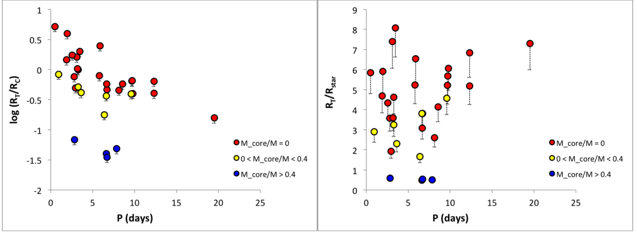
Fig. 12. Estimated ratios of truncation-to-corotation radius ( R_T/R_C , left ) and truncation-to-stellar radius ( R_T/R_\star , right ), as a function of rotation period for a subsample of CTTS in NGC 2264 with period measurements from this study and stellar and accretion parameters measured from Venuti et al. (2014). The estimates of R_T and R_C are obtained following Bessolaz et al. (2008), in the assumption that steady accretion funnels are formed. Circles correspond to truncation radius estimates obtained assuming that the sonic Mach number at the disk midplane ( m_s ) is equal to 1; the lower bar associated with each point marks by how much the values of R_T or R_T/R_C would vary if we adopted m_s = 0.5 (see Bessolaz et al. 2008). Red is used for objects with a mass ratio M_{\text{core}}/M_\star between the radiative core and the total mass of the star equal to 0 (i.e., fully convective objects); yellow identifies objects in the 0 < M_{\text{core}}/M_\star < 0.4 group; blue is for objects with M_{\text{core}}/M_\star > 0.4 . Different dipolar field strengths are used in the computation of R_T for each of these groups (see text).
