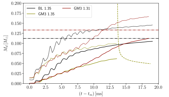
FIG. 7. Time evolution of disk mass for our simulations. The solid thick lines show the disk mass measure M_d , and the thin solid lines show the alternative measure M_d^{\text{alt}} . After the BH formation for model GM3 – 1.35, we show the mass outside the apparent horizon instead (dashed line). The rapid initial decrease corresponds to the rapid initial growth of the apparent horizon. The horizontal lines mark a disk mass for which the remaining remnant mass is at the upper limit for a SMNS (the two GM3 models are indistinguishable due to almost identical total mass).
