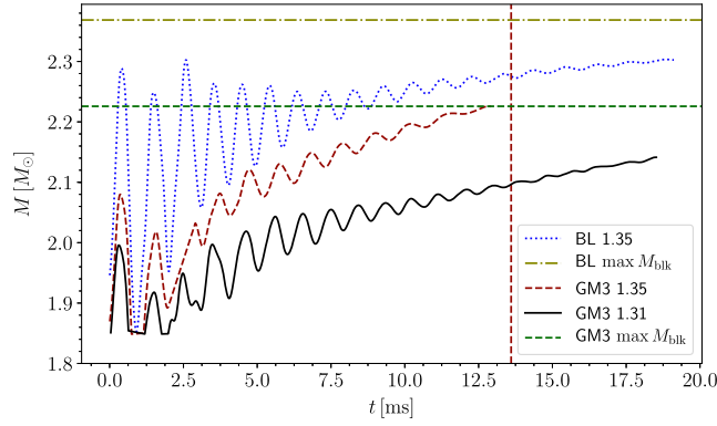
FIG. 9. Time evolution of the TOV solutions equivalent to the remnant cores (see text) for our simulations. The curves show the bulk mass of the TOV solutions, and the horizontal lines mark the maximum bulk mass for TOV sequences of the given EOS. The vertical line marks the BH formation.
