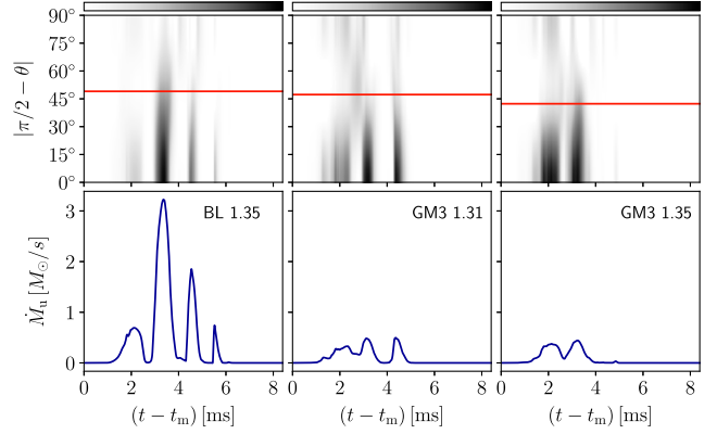
FIG. 12. Time evolution of the unbound matter flux through a spherical surface at r = 148 Km. Top panels: polar distribution of the flux reconstructed from the multipole moments up to l = 4 . The orbital plane corresponds to 0^\circ and the orbital axis to 90^\circ . The color scale is linear, ranging from zero (white) to the maximum flux for the given model (black). The horizontal line marks the angle below which 90% of the matter is ejected during the whole evolution. Bottom panels: total flux through the spherical surface, showing the contribution of the separate ejecta waves.
