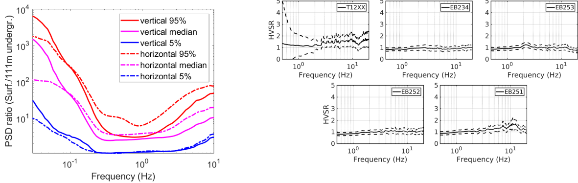
Figure 4. Horizontal-to-Vertical spectral ratio from active seismic measurement: peaks indicate resonance effect, but are significant only when amplitude is higher than 2.
