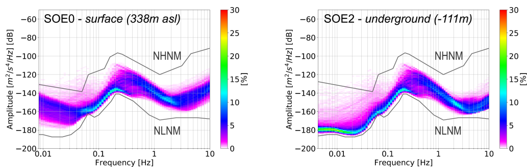
Figure 1. Power spectrum percentiles of seismic noise at Sos Enattos (vertical component), for the period April-August 2019. Left: surface measurement. Right: underground measurement below 111 m of rock. The continuous lines represents the Peterson models [6].
