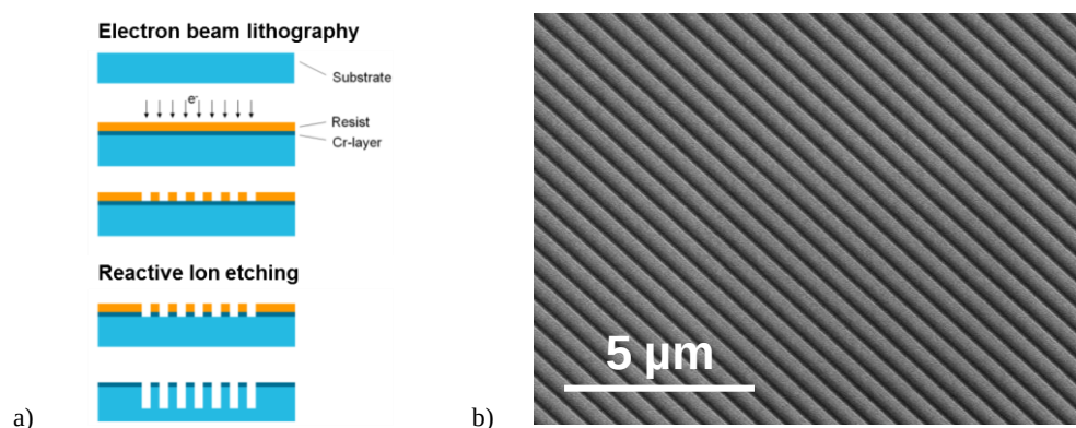
Figure 1. a) Fabrication process for binary surface relief gratings b) Scanning electron micrograph of a realized grating with 543 nanometers period ( \sim 1840 l/mm)
