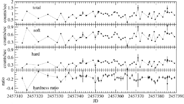
Figure 4. X-ray light curves of NGC 7469 in the hard (2.0–10.0 keV), soft (0.3–2.0 keV), and full bands. The light curve of the hardness ratio HR = (H - S)/(H + S) is also plotted.
