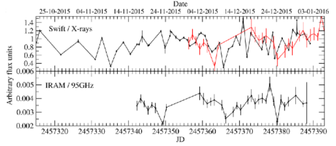
Figure 5. Light curves of NGC 7469 in X-rays (top) and 95 GHz (bottom). A tentative 14 day lag is demonstrated in the top panel by the red points, which are the (scaled) 95 GHz light curve shifted forward by 14 days.
