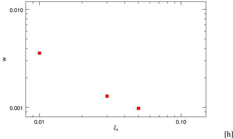
Fig. 5. Transverse size of the emission region as a function of \xi_e .
