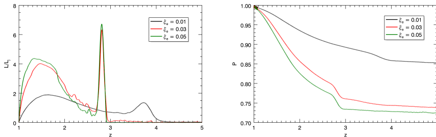
Fig. 6. The left panel shows the observed emissivity integrated over planes normal to the z axis as a function of the z coordinate. The right panel shows the energy flux integrated over planes normal to the z axis as a function of the z coordinate.
