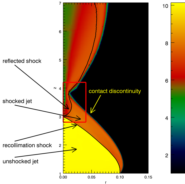
Fig. 1. Distribution of the Lorentz factor for the case with \xi_e = 0.01 , showing the main features of the steady solution. The red rectangle individuates the region shown in Fig. 2. Notice that the radial scale is strongly stretched.
