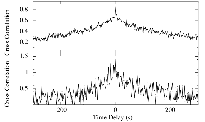
Fig. 8. z -transformed discrete correlation functions ( z DCFs) between the light curves of J1109 extracted in the soft and hard X-ray energy bands from XMM-Newton EPIC pn (top panel) and NuSTAR FPMA+FPMB (bottom panel) data using a time step of 2 s (see Sect. 6.2.1 for the definitions adopted for the energy bands). The z DCFs have been normalised so as to account for Poisson noise. Positive time delays correspond to higher energy photons lagging lower energy photons. For plotting purpose, an extended range of time delays is shown, and uncertainties on the values have been omitted.
