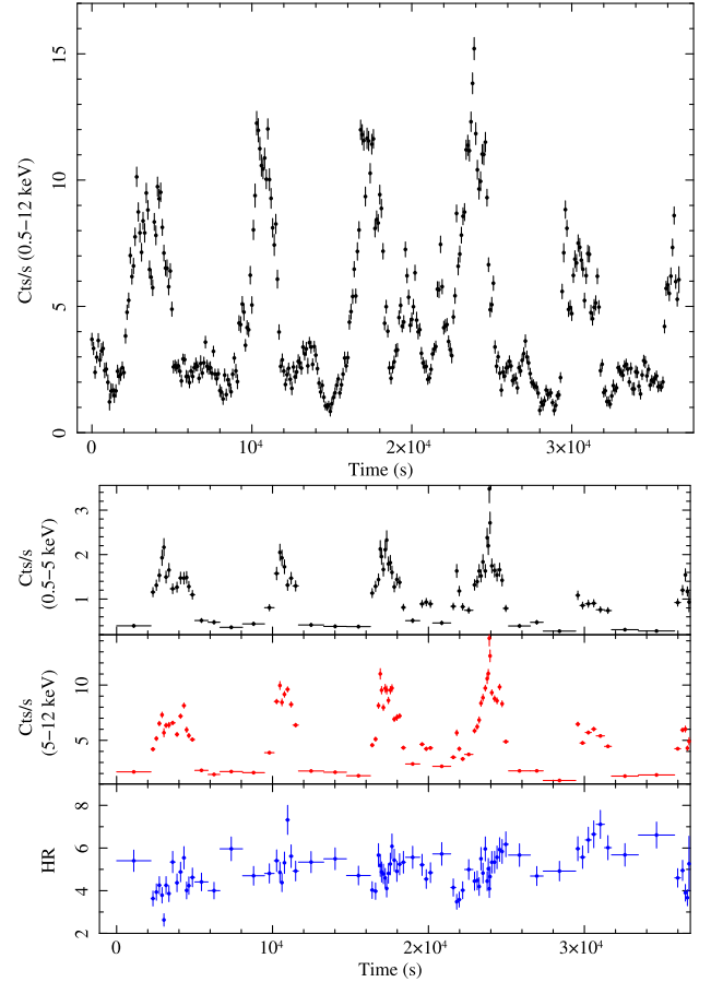
Fig. 4. Top: 0.5–12 keV pn light curve of IGR J17329-2731 with a time resolution of 100 s. Bottom: the energy-resolved pn light curve of IGR J17329-2731 (top and middle panels) and the correspondingly computed HR (bottom panel).
