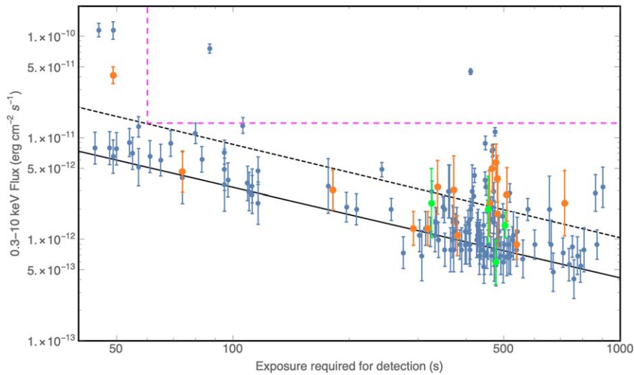
Figure 3. Plot of the peak fluxes of all sources vs. the theoretical exposure time required to detect each source. The black solid/dashed lines represent the XRT sensitivity as a function of exposure time, at the 50%/90% confidence levels (from 1SXPS), respectively (note that the sensitivity “lines” are rather curves, since they are shown in log space). The plotted points represent the peak fluxes of each source (with their corresponding 1\sigma uncertainties; y-axis) vs. the effective exposure time needed to detect a source at its flux. Sources that exhibited slight fading ( 1 < \sigma \leq 2 ) are highlighted in orange, and sources that exhibited more significant fading (at least >2\sigma ) are highlighted in green (though these sources all have >4\sigma significance). Some sources have exposures for detection >560 s, which were found in the overlapping regions of adjacent tilings. The two sources fully enclosed within the dashed pink dashed lines are sources not detected in the initial 60 s exposures, but they should have been had they been this bright (i.e., at their peak flux) when those observations were carried out.
