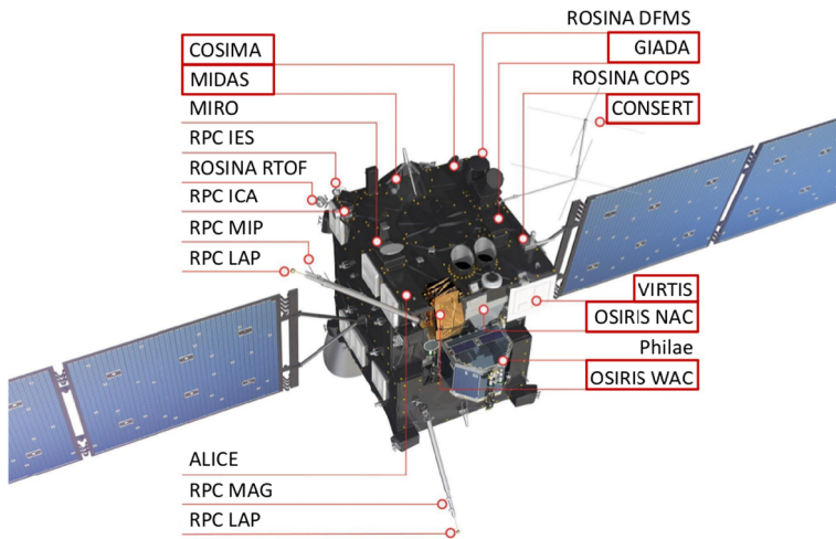
Fig. 1 Rosetta with labelled instruments, including the lander before its release. The dedicated dust analysing instruments COSIMA, GIADA and MIDAS, as well as the OSIRIS camera system, the VIRTIS VIS/NIR imaging spectrometer and the CONSERT antenna are located on the panel of Rosetta that is mainly oriented towards the cometary nucleus. After ESA/ATG medialab
