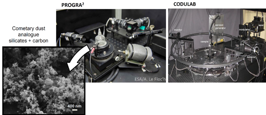
Fig. 8 Instruments PROGRA 2 (Hadamcik et al. 2009a) and CODULAB (Muñoz et al. 2011), used to measure, through experimental studies in the laboratory or under microgravity conditions, the light scattering properties of various analogues of cometary dust in suspension
