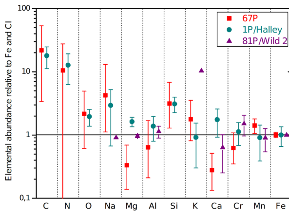
Fig. 2 Comet 67P/C-G dust elemental ratios relative to Fe and to the CI chondrite composition (Lodders 2010) compared to 1P/Halley's dust and 81P/Wild 2's dust collected in Stardust aerogel. The values correspond to the relative ratios (E/Fe)_{\text{comet}}/(E/Fe)_{\text{CI}} . The N/C atomic ratio has been measured by Fray et al. (2017). The error bars for 67P/C-G data come from the uncertainties on the determination of Relative Sensitivity Factors' (RSFs) uncertainties and can be amplified by successive normalizations. For instance, the uncertainty displayed for C is the addition of uncertainty on the RSF for calculation of C/Si, plus uncertainty for Si/Fe, plus uncertainty on C/Fe in CI-type chondrite. Therefore, error bars can be "artificially" enhanced due to successive normalizations to compare all elements on a same plot (this explains why error bars on N are so large in this plot, compared to the actual value measured for N/C = 0.035 \pm 0.011 (Bardyn et al. 2017))
