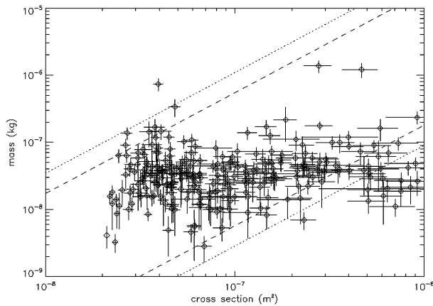
Fig. 6 Mass and cross-section measurements of compact particles detected by GIADA from August 2014 to September 2016 (the error bars refer to 1\sigma standard error of the 271 GDS+IS measurements). The data are compared with the trends of prolate and oblate ellipsoids of aspect ratio of 10 (dotted lines) and 5 (dashed lines), respectively, and with dust bulk densities of Fe sulphides, \rho_1 = 4600 \text{ kg m}^{-3} (upper lines), and of hydrocarbons, \rho_2 = 1200 \text{ kg m}^{-3} (lower lines). The GDS signal saturates at a cross section >10^{-6} \text{ m}^2 . Particles with cross-sections <2 \times 10^{-8} \text{ m}^2 (and most of those with mass <10^{-8} \text{ kg} ) were too small and fast to be detected by GDS. The flux at masses >2 \times 10^{-7} \text{ kg} was very low during the entire mission due to the spacecraft safety constraints. All these facts explain why all data are distributed in a mostly horizontal cloud. The particles close to the upper dotted and dashed lines have an almost zero porosity, and are compact aggregates of minerals condensed in the inner protoplanetary disc (they are too large to have an interstellar origin Brownlee 2014). The particles at right of the lower dotted and dashed lines have both a large porosity and a composition dominated by hydrocarbons. The particles in between are a porous mixture of minerals and hydrocarbons
