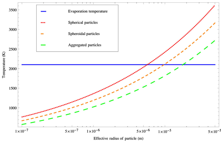
Fig. 10 Maximum equilibrium temperatures for particles entering the Earth atmosphere at 30 \text{ km s}^{-1} . The horizontal line corresponds to a typical temperature of sublimation of 2100 K (adapted from Levasseur-Regourd and Lasue 2011)
