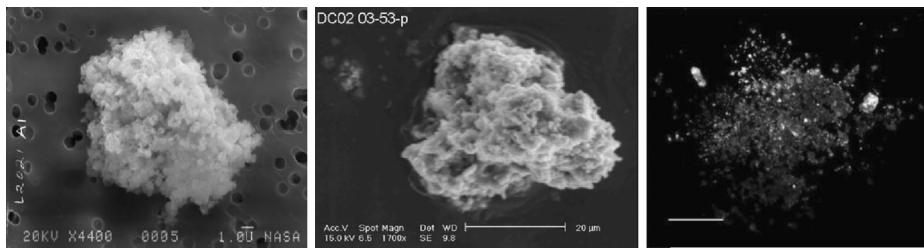
Fig. 9 From left to right, ordered by increasing sizes: Electron micrograph of stratospheric IDP (Particle L2021A1, about 13 \times 10 \mu\text{m} , credit NASA); Electron micrograph of Antarctic micrometeorite DC02-03-53 collected near the Concordia station (size about 30 \times 40 \mu\text{m} , Duprat et al. 2007); Optical image of the giant cluster IDP U2-20GCA (scale bar 100 \mu\text{m} ) Messenger et al. 2015)
