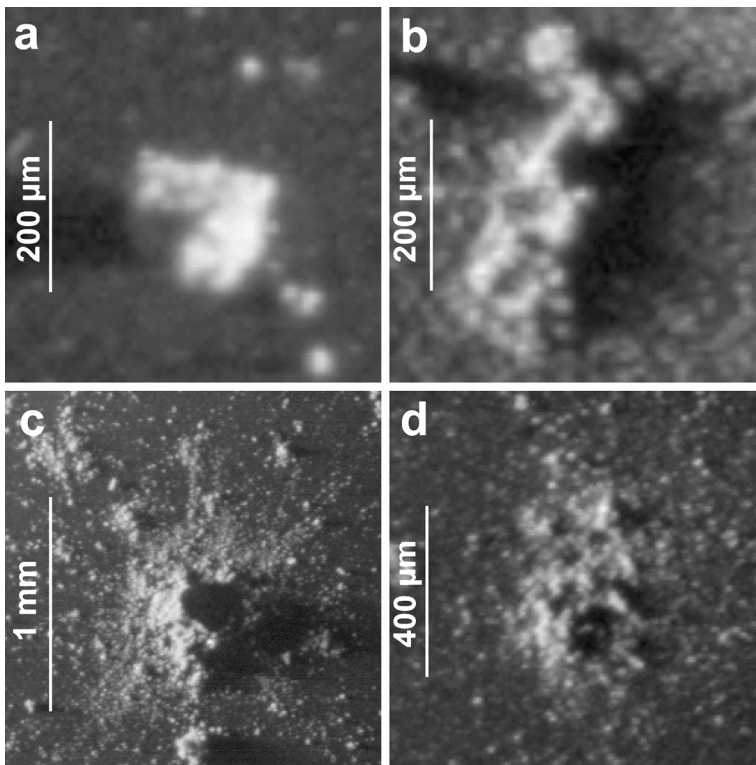
Fig. 5 Morphology of particles collected by COSIMA, using the classification of Langevin et al. (2016); (a) “compact” particle exhibiting well-defined boundary; (b) “glued cluster”, with sub-components apparently linked together by a matrix; (c) “rubble pile”, with a central mound surrounded by an apron of smaller sub-components; (d) “shattered cluster”, with widely distributed components and a size to height ratio smaller than 10. Such particles present morphological similarities with the largest particles collected by MIDAS (Fig. 4), which are 10 times smaller
