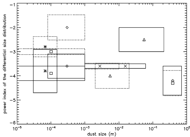
Fig. 7 Power index of the differential size distribution of 67P/C-G. Dotted lines: power index before the 2015 equinox. Continuous lines: power index after the 2015 equinox, up to just after the 2015 perihelion. The ranges along the x axis show the instrument sensitivity, the ranges along the y axis are given by the uncertainty of the power index. Stars: COSIMA data (Merouane et al. 2017). Diamonds: GIADA data (Rotundi et al. 2015; Fulle et al. 2016c). Triangles: OSIRIS observations of single particles in the coma (Rotundi et al. 2015; Fulle et al. 2016c; Ott et al. 2017). Dotted diamond: OSIRIS observations of pebbles in Sais (Pajola et al. 2017a). Dotted square: ROLIS observations of pebbles in Agilkia (Pajola et al. 2017a). Squares: Ground-based observations, tail models (Moreno et al. 2017). Crosses: Ground-based observations, trail models (Moreno et al. 2017)
