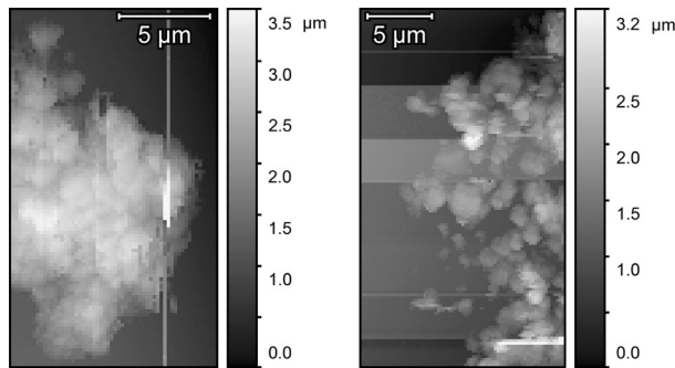
Fig. 4 Left panel: A typical compact particle collected with MIDAS, extending beyond the field of view and exhibiting a well-defined boundary. The surface features at smaller scales are interpreted as individual units composing the dust. Right panel: A large fluffy particle (also extending beyond the field of view of MIDAS) that is interpreted to represent the remains of a fractal aggregate with fractal dimension D_f = 1.7 \pm 0.1 that compacted on collection (Mannel et al. 2016). Another possibility, the rebound of a larger dust particle bouncing on the target and depositing a surface layer, is less likely due to the structural differences found in experimental tests (Ellerbroek et al. 2017). ESA/Rosetta/IWF for the MIDAS team IWF/ESA/LATMOS/Universiteit Leiden/Universität Wien
