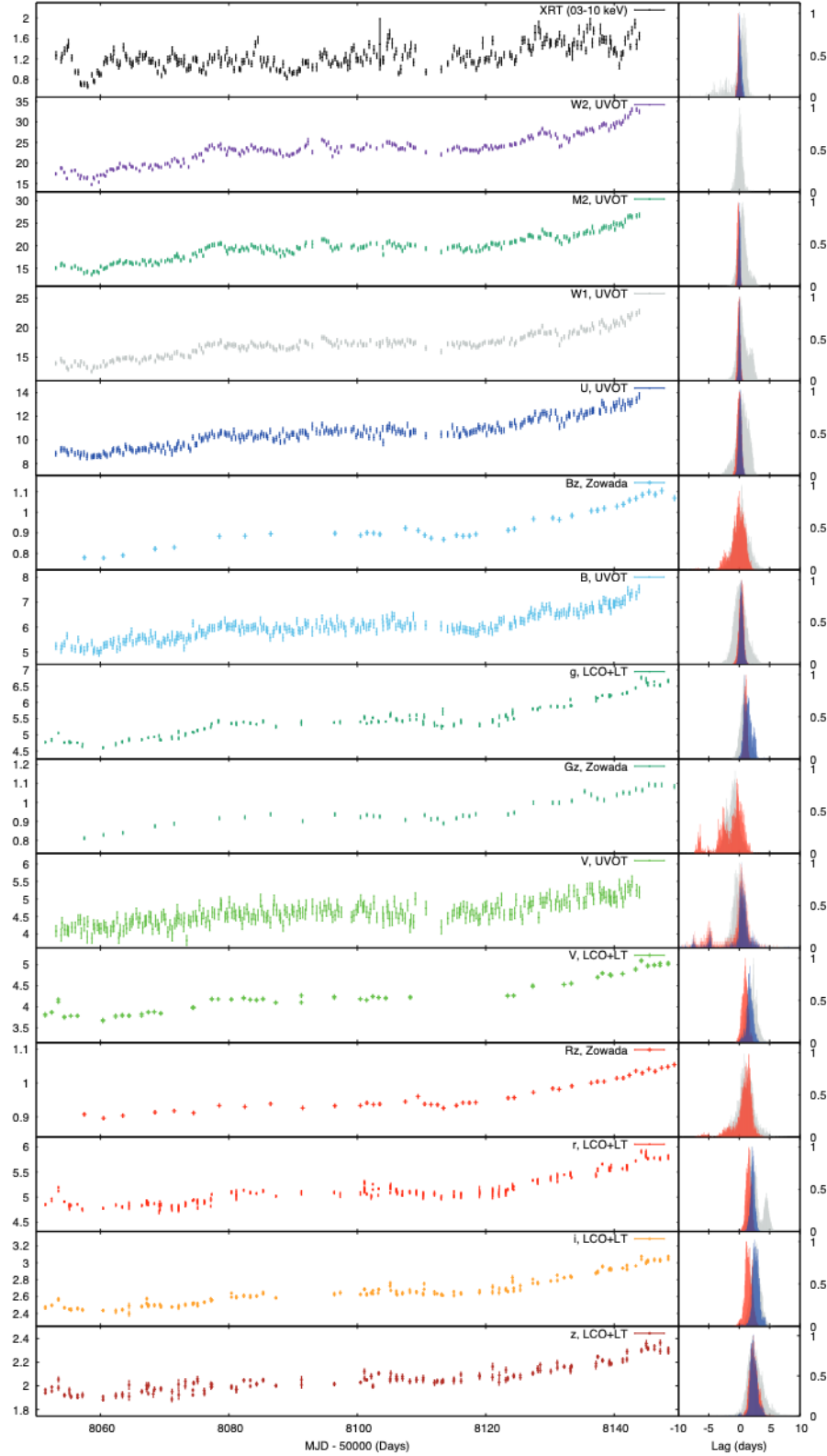
Figure 2. Left-hand panels: Light curves used for the short time-scale lag analysis. While the XRT light curve is shown in count s^{-1} , the measurements in the UVOT filters are in (\times 10^{-15}) \text{erg cm}^{-2} \text{s}^{-1} \text{\AA}^{-1} . Regarding the ground-based observations, LCO + LT is in (\times 10^{-15}) \text{erg cm}^{-2} \text{s}^{-1} \text{\AA}^{-1} , while RGB Zowada light curves are in arbitrary units. Right-hand panels: Lag versus UVW2 band probability distribution using unfiltered light curve (grey), and filtered ones by removing the linear trend (red) and a 10-d box-car moving average (blue).
