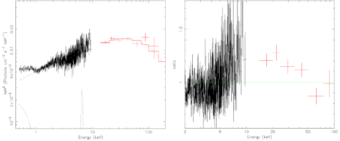
Figure 9. Left-hand Panel: X-ray emission spectrum observed by Swift XRT (black points) and BAT (red points) and modelled with MODEL 1. Right-hand Panel: Ratio of the data to a simple power-law model.
