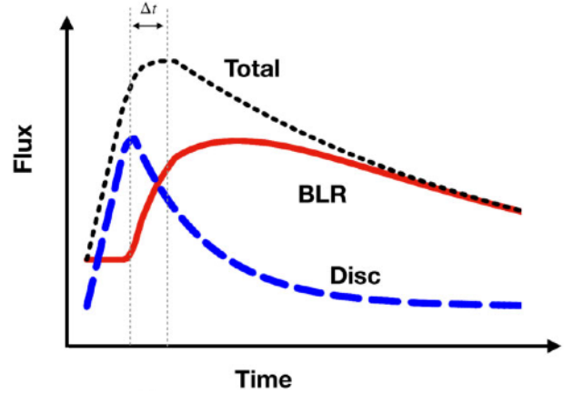
Figure 11. Diagram of the proposed physical scenario for the observed long term trend in the optical bands (black fine-dashed curve), assuming a linear rise and an exponential decay. If we assume that the BAT flare is driven by the disc emission (blue long-dashed curve), then this has a similar rise, an earlier peak (peaks separated by \Delta t ), and a faster decay than the optical bands. Therefore, in order to recover the total light curve, an additional component is needed. We interpret the difference between the total and the disc light curve as the contribution from the DC (red curves), which dominates the emission after the peak.
