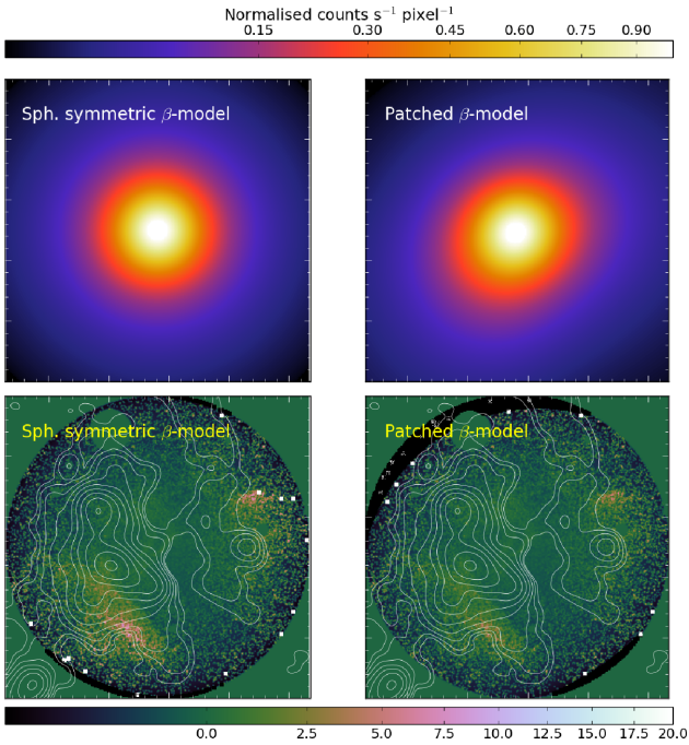
Figure 9. Top panels: Normalized spherically symmetric \beta -model (left) and patched \beta -model (right) used to derive a first-order density gradient of the gas. Bottom panels: residuals of the X-ray emission after division by the spherically symmetric \beta -model (left) and patched \beta -model (right).
