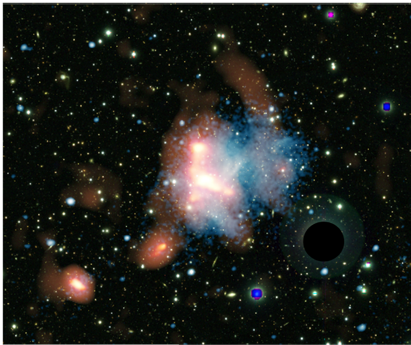
Figure 2. Subaru b , v , and z composite image overlaid on to X-ray emission from Chandra (cyan) in the band 0.2–5 keV, and radio emission from LOFAR at 147 MHz (orange). The image has illustrative purposes only. A black circle is superposed on a bright star to mask it. Quantitative values for the X-ray and radio emission are shown in Figs 1 and 3, respectively.
