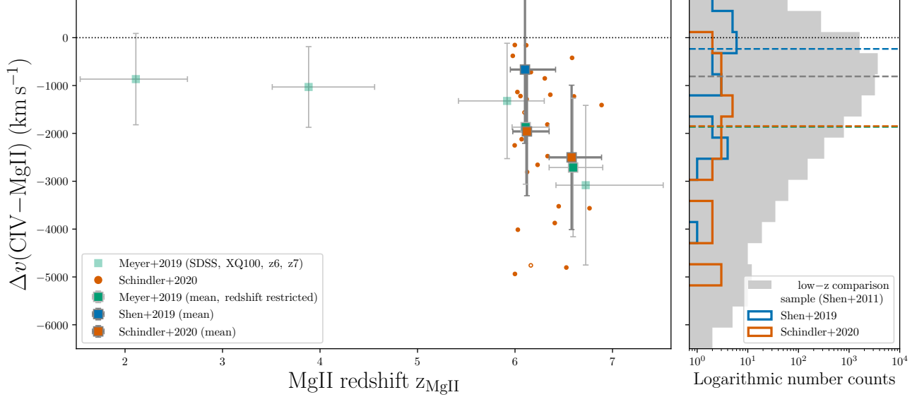
Figure 11. Left panel: CIV-MgII velocity shifts of individual high-redshift quasars as a function of the Mg II redshift. Our results are shown in orange. We calculate the mean (orange square) and standard deviation (dark grey error bars) CIV-MgII for two sub-samples split at z = 6.35 . The error bars in the redshift direction show the redshift bin. We contrast these results with the mean results of the samples of Meyer et al. (2019) (light green squares). For an appropriate comparison we restrict the z6 and z7 Meyer et al. (2019) samples to the same redshift ranges as our sample and re-compute the mean (green squares), yielding very good agreement with our data. All velocity shift measurements are based on the peak redshifts of the emission lines. Right panel: Logarithmic CIV-MgII velocity shift histograms. We compare our results (orange) to the high-redshift sample of Shen et al. (2019a) (blue). Both measurements are contrasted with low redshift data from Shen et al. (2011) at 1.5 \leq z \leq 2.2 and restricted to \log(L_{\text{bol}}/\text{erg s}^{-1}) = 46.5 - 47.5 for a valid comparison to the high redshift quasars. The colored dashed lines show the median of the three distributions as well as the combined z6 and z7 samples of Meyer et al. (2019) (green).
