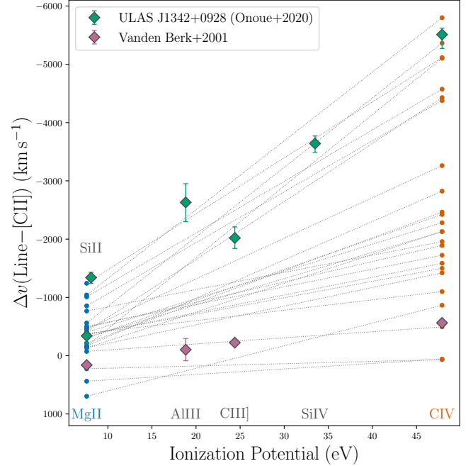
Figure 15. Velocity shifts of emission lines as a function of ionization potential. We only show show Mg II-[C II] 158 μm and C IV-[C II] 158 μm velocity shifts of quasars of our sample with solid blue and orange points. Measurements of the same quasar are connected with a dotted grey line. We compare these measurements with various velocity shifts from ULAS J1342+0928 (Onoue et al. 2020), which were also measured with respect to [C II] 158 μm in green. The purple data points show velocity shifts with respect to [O III] 5007 Å from the low-redshift quasar composite of Vanden Berk et al. (2001). Quasars from our sample show a large range of blueshifts.
