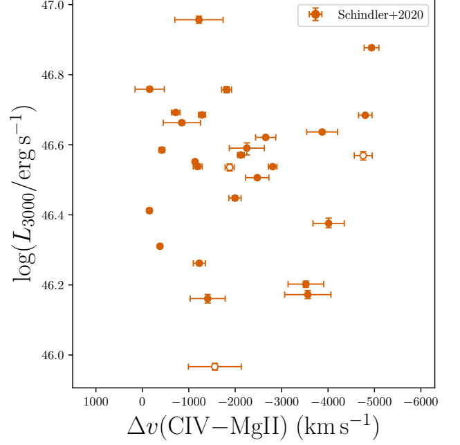
Figure 17. Luminosity at 3000 Å as a function of the C IV-Mg II velocity shift for quasars in our sample. Our sample does not show a correlation between continuum luminosity and C IV-Mg II blueshift.
