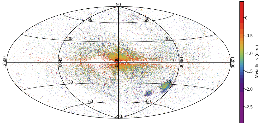
Fig. 34. Same as in Fig. 33, but showing only 88 440 RR Lyrae stars with an error in metallicity \sigma_{[\text{Fe}/\text{H}]} \leq 0.46 dex.
