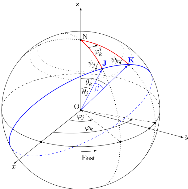
Fig. A.1. Definition of points and angles on the sphere involved in the geometry of the smoothing of polarization maps (adapted from Keegstra et al. 1997). J is the position of the centre of the smoothing beam, and K a neighbouring pixel, with spherical coordinates (\varphi_*, \theta_*) and (\varphi_k, \theta_k) , respectively. The great circle passing through J and K is shown in blue. The position angles \psi_* and \psi_k here are in the HEALPix convention, increasing from Galactic north toward decreasing Galactic longitude (west) on the celestial sphere as seen by the observer at O.
