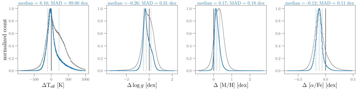
Fig. 13. Comparison of the APs from GSP-Spec-Matisse Gauguin and ANN for the Gaia DR3 sample with the first 13 and 8 values in astrophysical_parameters.flags_gspspec and astrophysical_parameters_supp.flags_gspspec_ann equal to zero. This represents 1 084 427 stars in the Gaia DR3 catalogue. For reference, we also indicate the distribution without the flag filtering in grey.
