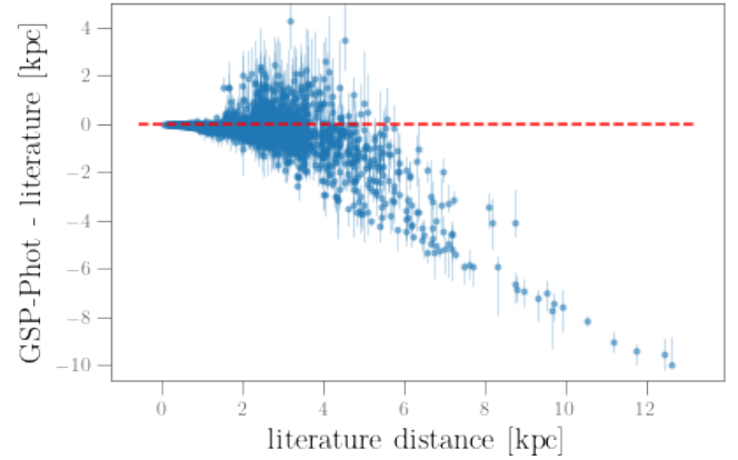
Fig. 7. Comparison of GSP-Phot distances in star clusters against literature values. For 2019 star clusters (nearly 200 000 stars) spanning distances up to 13 kpc, we indicate on the y-axis the median offset (dot), and the 50% quantile (line) of all member star distances with respect to cluster distances taken from Cantat-Gaudin et al. (2020). Above \sim 2.5 kpc ( \sim 15\% of the cluster members), GSP-Phot systematically underestimates distances (see the discussion Sect. 3.1).
