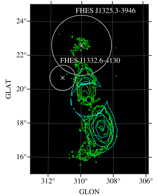
Figure 6. Map of the Cen A region, showing contours for the LAT \gamma -ray Cen A Lobes template (cyan) and Parkes radio continuum map at 5 GHz (green). The white circles with central marker \times indicate the best-fit disk radius and centroid of the two FHEs sources associated with Cen A: FHEs J1325.3-3946 and FHEs J1332.6-4130.
