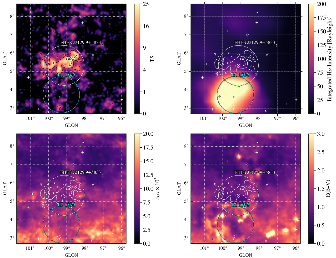
Figure 10. TS map of FHEs J2129.9+5833 (top). The top right plot shows the velocity-integrated map of H_{\alpha} from the WHAM Sky Survey, with the LAT TS isocontours overlaid. Bottom panels show maps of Planck dust optical depth at 353 GHz (left) and SFD dust reddening (right), with LAT TS isocontours overlaid. The white circle with central marker \times indicates the best-fit disk extension and centroid of the FHEs source. White crosses indicate the positions of point-source candidates with TS > 9 from the best-fit model for the region. The LAT TS isocontours are also shown in white. Green crosses indicate the positions of sources in the 3FGL catalog. The cyan circle indicates the location of the H II region IC 1396.
