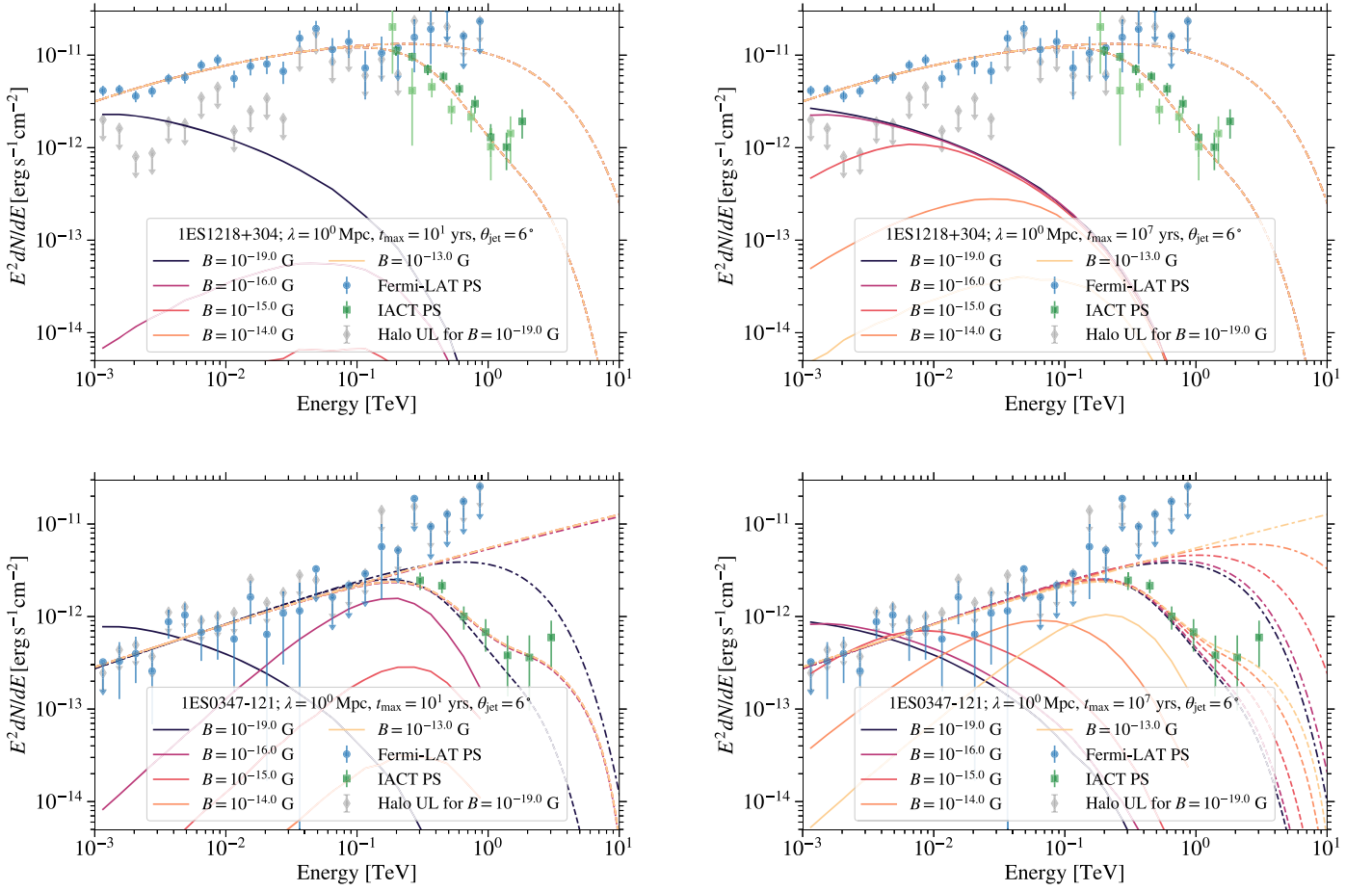
Figure 19. Same as Figure 18 for the TeV detected blazars 1ES 1218+304 and 1ES0347-121 that yield constraints on the IGMF.
