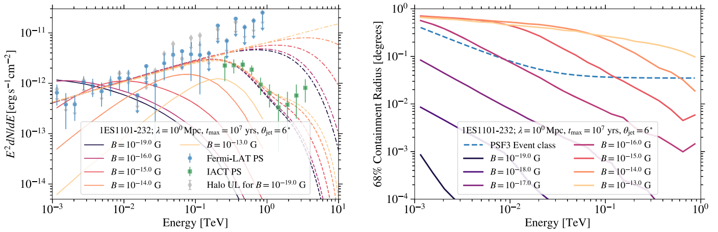
Figure 16. Left: fit of the intrinsic spectrum and cascade component to the IACT and Fermi -LAT data of 1ES 1101-232 ( z = 0.186 ) for different IGMF strengths. A source activity time of t_{\max} = 10^7 years and a jet opening angle of \theta_{\text{jet}} = 6^\circ are assumed, along with a coherence length of 1 Mpc. The best-fit intrinsic spectra multiplied with EBL absorption are shown as dashed lines with colors matching those of the cascade component (solid lines). The intrinsic spectra are shown as dash-dotted lines. Upper limits on the halo energy flux for widths equal to that of the cascade for B = 10^{-19} G are shown as gray diamonds. Right: containment radii for the cascade ( R_{\text{casc}} ) for different B -field strengths and the PSF (PSF3 event class) as a function of energy for the same source and parameters as the right panel. We show the containment radii for two additional B -field strengths ( 10^{-18} G and 10^{-17} G) compared to the left panel to better illustrate the IGMF dependence on this quantity. The spectra for these values of B would be very similar to the ones shown for 10^{-19} G or 10^{-16} G.
