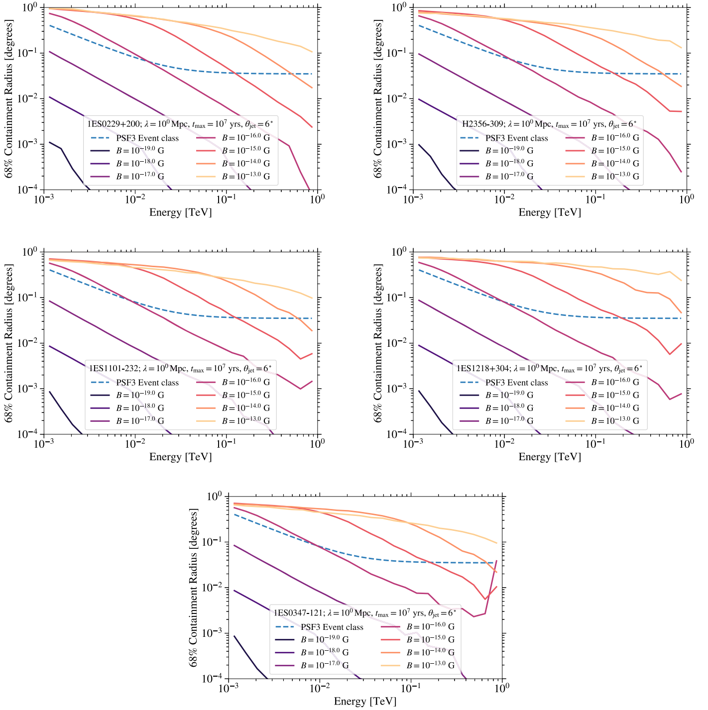
Figure 20. Same as Figure 16 (right) for the TeV-detected blazars that yield constraints on the IGMF, assuming a maximum activity time of t_{\text{max}} = 10^7 years.
