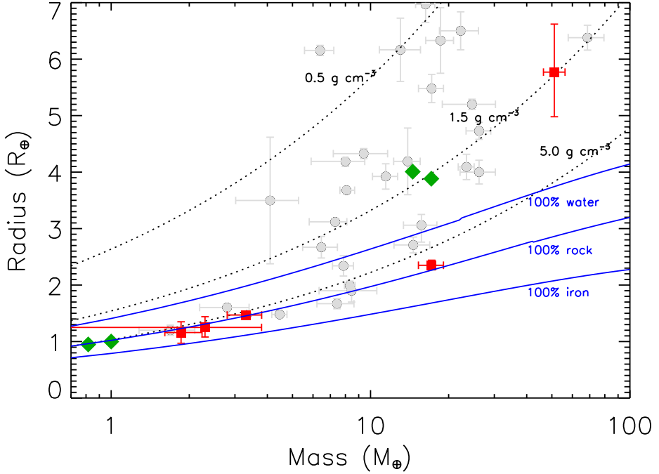
Fig. 1. Mass-radius diagram of the known transiting planets with radius R_p \leq 7 R_{\oplus} , mass M_p \leq 100 M_{\oplus} , and precision on the mass better than 30%. Green diamonds indicate Neptune, Uranus, the Earth, and Venus (from right to left). The three dotted lines indicate isodensity curves of 0.5 , 1.5 , and 5 \text{ g cm}^{-3} , and the blue solid lines show the mass and radius of planets consisting of pure water, 100% rocks, and 100% iron Seager et al. (2007). The positions of the Kepler planets characterized with HARPS-N to date are shown with red squares.
