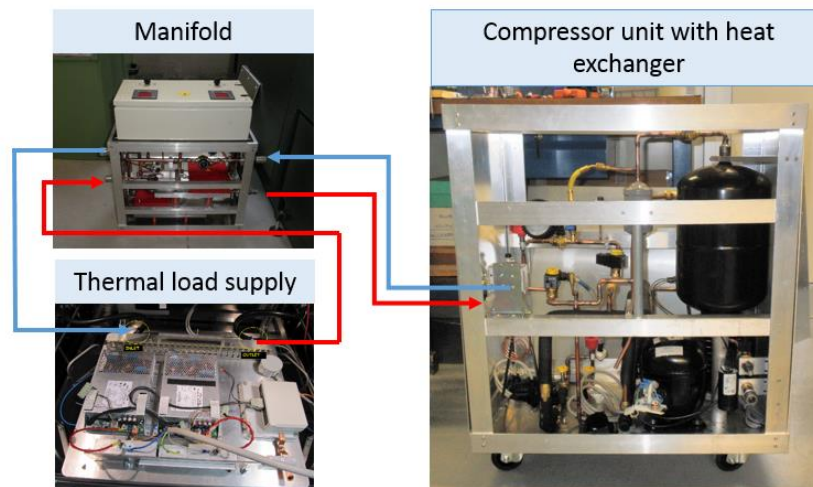
Figure 13. Experimental setup.
