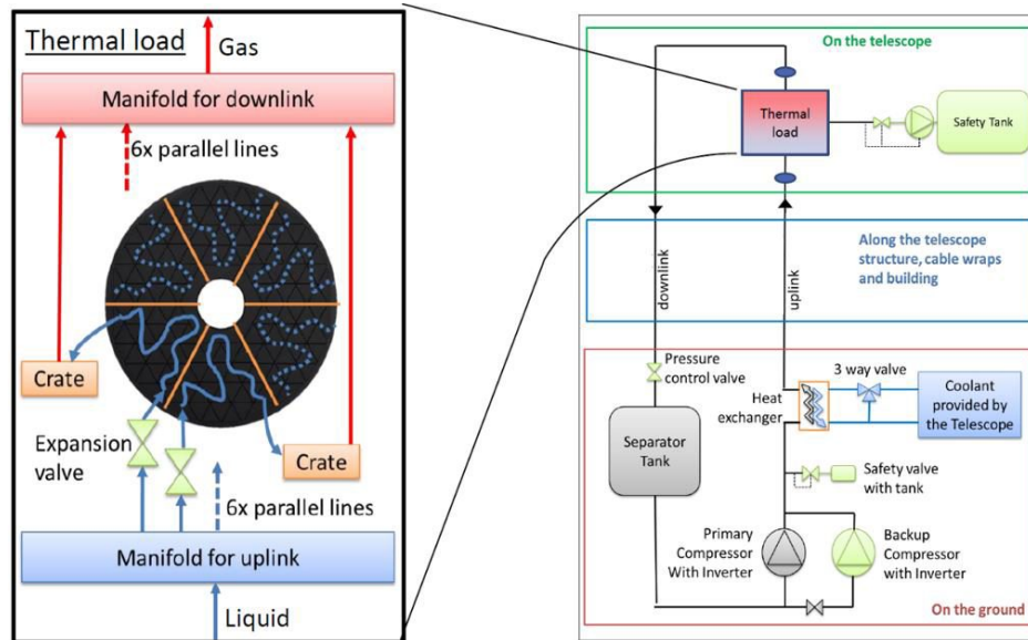
Figure 11. Expansion gas cooling layout of the E-ELT M4.
