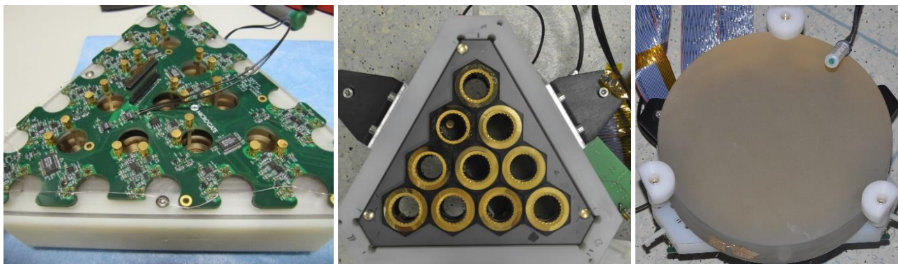
Figure 8. BB5 electronic board (left), SiC reference body with metalized tiles (center), coated Clearceram-Z mirror (right).
