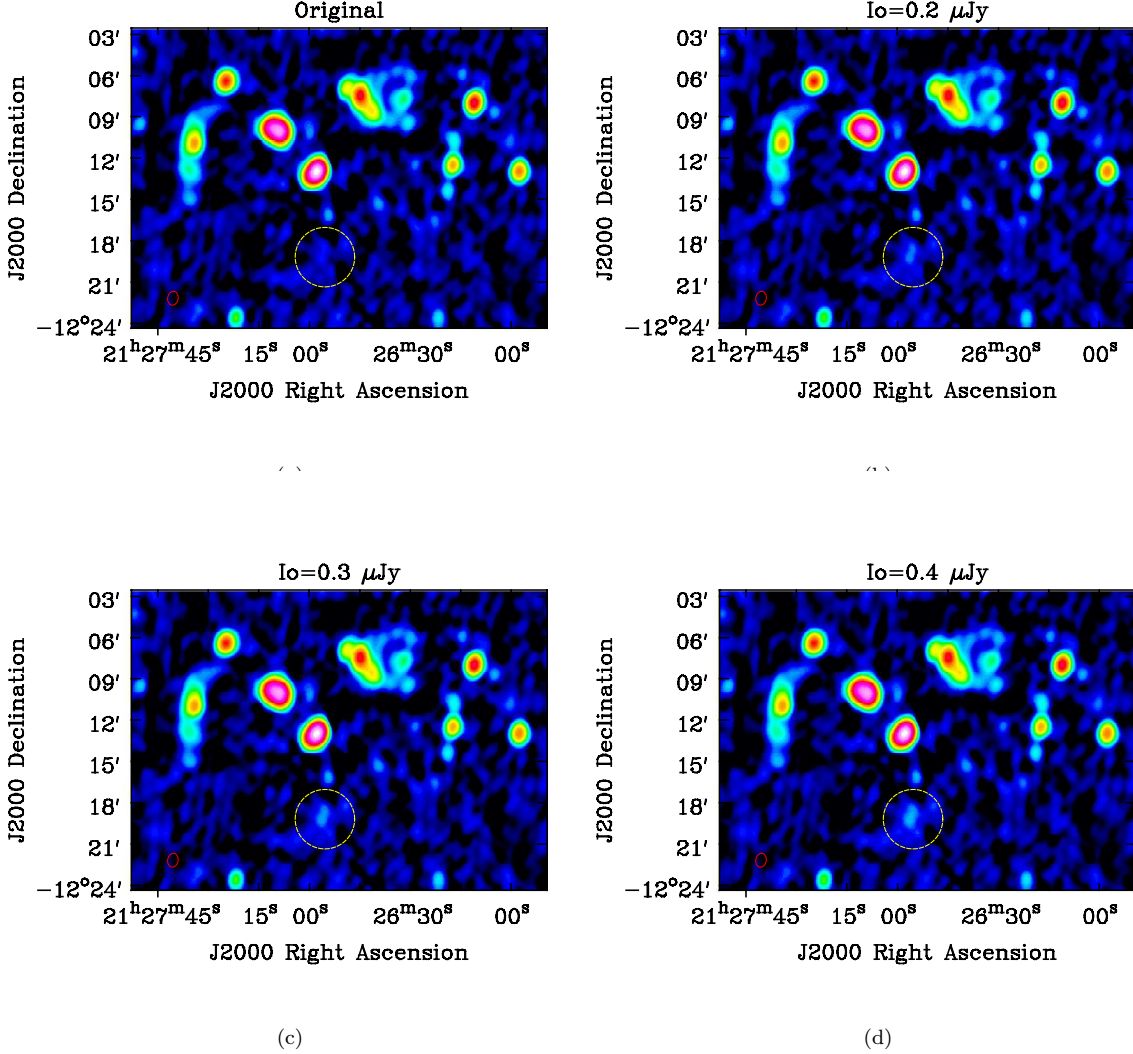
Figure 1. Mock halos in the cluster A2345. Images of the cluster (a): original dataset, (b): mock halo with I_0 = 0.2 \mu\text{Jy/arcsec}^2 (c) mock halo with I_0 = 0.3 \mu\text{Jy/arcsec}^2 (d) mock halo with I_0 = 0.4 \mu\text{Jy/arcsec}^2 . The yellow circle is centred on the halo and has a radius r = R_H . The images have been obtained with the same parameters, and displayed with the same color scheme. The mock halo that fulfils the criteria for detection is the one in panel (c)
