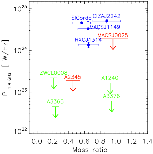
Figure 6. P_{1.4\text{ GHz}} versus the merger mass-ratio. Blue points are detected halos, red arrows are upper limits below the P_{1.4\text{ GHz}} - M_{500} correlation, green arrows are upper limits above the P_{1.4\text{ GHz}} - M_{500} correlation. As errors on the masses of the sub-clusters are not available for most objects, we assume a fiducial error of 20% on the mass ratios.
