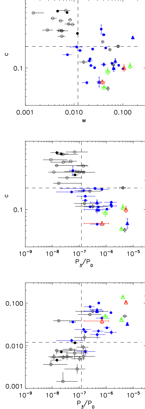
Figure 4. Morphological estimators of cluster dynamical status from X-rays. Black filled dots are clusters with mini halos, blue filled dots are clusters with radio halos and no double relics (from Cassano et al. 2010; Venturi et al. 2008; Bonafede et al. 2014, 2015), blue filled triangles are clusters with radio halos and double relics, red open triangles are clusters with double relics and no radio halo (upper limit below the P_{1.4\text{GHz}} - M_{500} correlation), black spheres are clusters with no radio halos and no double relics. Green triangle mark clusters where no radio halo has been detected but the upper limit is above the P_{1.4\text{GHz}} - M_{500} correlation. Dashed lines are the median of the parameters, that define radio-loud and radio-quiet quadrants (Cassano et al. 2010)
