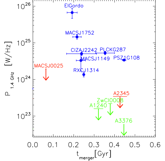
Figure 7. P_{1.4\text{ GHz}} versus estimate of the time-since-merger. Blue points are detected halos, red arrows are upper limits below the P_{1.4\text{ GHz}} - M_{500} correlation, green arrows are upper limits above the P_{1.4\text{ GHz}} - M_{500} correlation.
