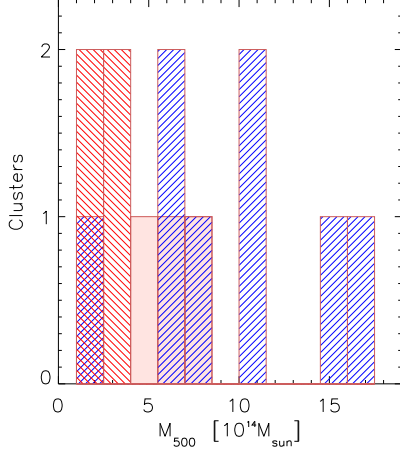
Figure 5. Histogram of the clusters with halo (blue diagonal lines), without halo (filled red), and with upper limit consistent with the P_{1.4\text{ GHz}} - M_{500} correlation (red diagonal lines) versus the cluster mass.
