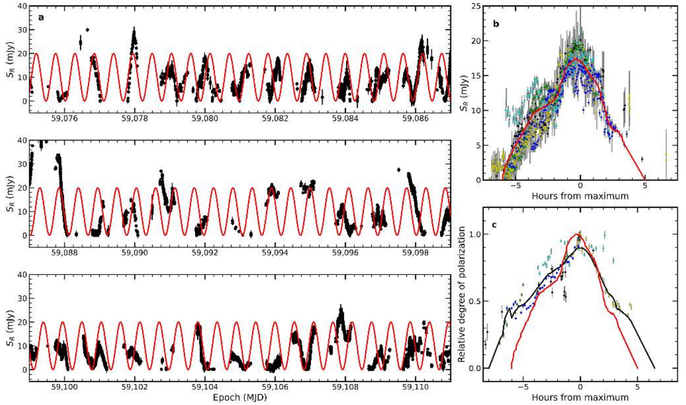
Extended Data Fig. 7 | QPOs in optical R -band flux density. a , Oscillations in optical R -band flux density during the outburst over the time interval 13 August 2020 to 18 September 2020 ( n = 8,106 ), with the long-term trend subtracted. For comparison, the red curve represents a sinusoidal function with a period of 0.55 days and an amplitude of 20 mJy. b , Average profile of the optical flux
