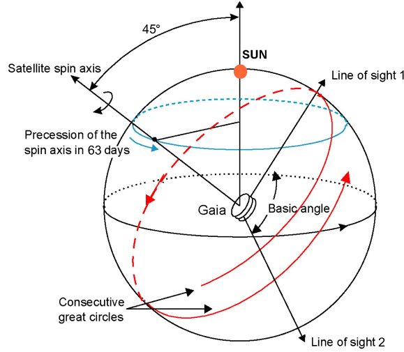
Fig. 4. – Gaia measurement principle. Credit: ESA
