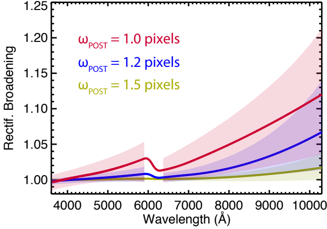
Figure 8. Effective LSF broadening factor (i.e., the ratio of the post-pixellized LSF in units of Å measured before and after rectification) introduced by the spectral rectification of the native-pixel blue and red camera spectra onto a fixed logarithmic wavelength grid. Solid red, blue, and gold lines show the median broadening as a function of wavelength computed via Monte Carlo analysis of artificial spectra for input widths of \omega = 1.0, 1.2 , and 1.5 pixels respectively. In each case the shaded region shows the 1\sigma variation about the mean traced by input lines with different effective pixel phases. The corresponding curves for the linear wavelength grid (not shown) are generally similar except in the 9000 - 10,000 Å range where the logarithmic output grid undersamples the typical input LSF.
