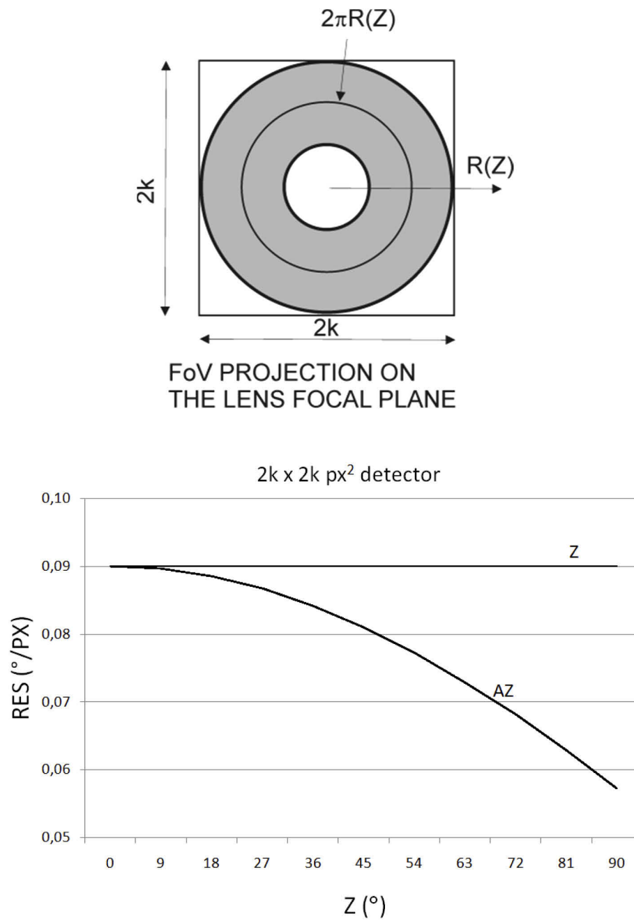
Fig. 5. Z and AZ image forming (top) and resolution ( ^{\circ}/px ) of the lens considering a 2k \times 2k image sensor (bottom).
