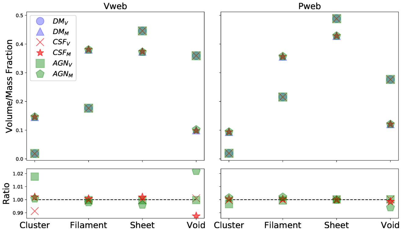
Figure 4. Upper panel: the volume and mass fractions of the structures. Lower panel: respective ratios between the CSF/AGN and DM-only runs. Left-hand column shows the results from the vweb code, while the right-hand column is for the pweb code. The meaning of the symbols is shown in the legend on the top left-hand panel, where sub-indexes V and M indicate volume and mass fractions.
