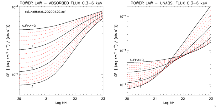
Fig. 37 SXI counts to flux conversion rates for a power-law spectrum as a function of absorption. The lines refer to different values of the photon index. The left figure refers to absorbed fluxes and the right one to fluxes corrected for the absorption.
