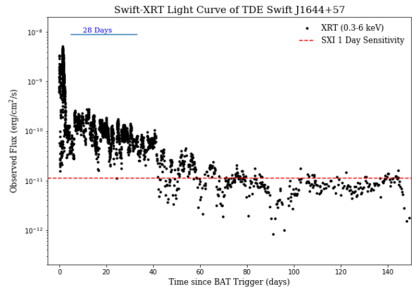
Fig. 32 Observations of the hard TDE Swift J1644+57. The red dashed line shows the detection limit for each pointing of approximately 2.3 ks several times a day with the SXI (0.2–6 keV). It is obvious that a highly detailed lightcurve can be obtained of a similar event.
