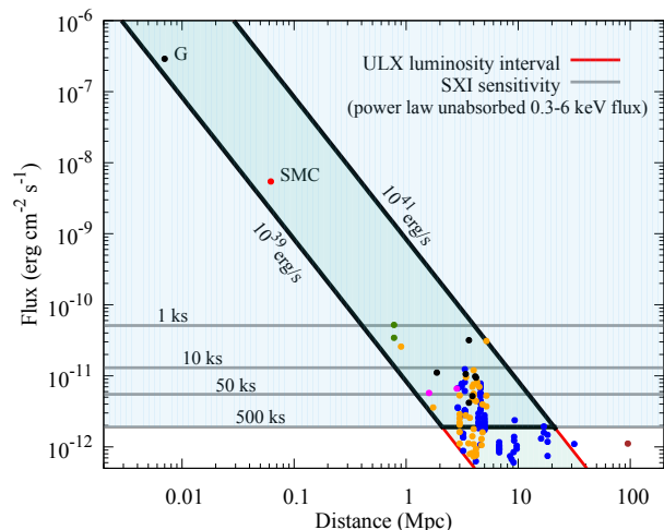
Fig. 24 Estimate of the region in the flux vs. distance plane where SXI can detect the potential sources within the standard ULX luminosity interval ( 10^{39} – 10^{41} \text{ erg s}^{-1} ). The SXI sensitivity (unabsorbed 0.3–6 keV flux) delineated by the horizontal gray lines labeled with minimum exposure times intersect with the ULX luminosity interval determined by the oblique red lines to define the region for the potential ULX targets THESEUS can monitor. The shaded green area bounded by the solid black curve displays such a sample region where ULXs with standard luminosities can be detected and monitored by SXI for an integration time of \leq 500 ks. Filled circles with different colors represent the observed ULXs from different catalogs/references: [214] blue; [215] orange; [126, 207, 209, 210, 211] black; [216, 217] green; [218] red; [219] magenta; [220] brown. As the spectral energy range for each source group does not perfectly match the energy range of SXI and the spectral model for each source may differ from a pure power law, the source distribution is an approximation to the actual population of ULXs SXI can detect. The two nearest ULXs are marked by G (Galactic) and SMC (Small Magellanic Cloud) labels.
