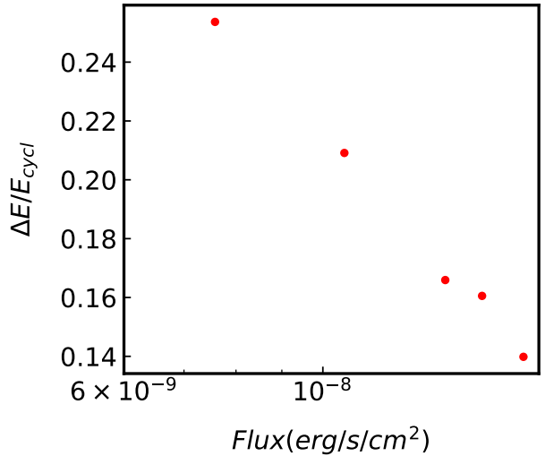
Fig. 15 Relative error (90% c.l.) on the determination of the cyclotron line energy as a function of source observed flux (2-200 keV) for simulated XGIS observations of 70 ks exposure time. We used a spectrum as observed in HMXB Cen X-3 [111], consisting of exponentially cut-off power law with an absorption line at E_c = 30.7 keV.
