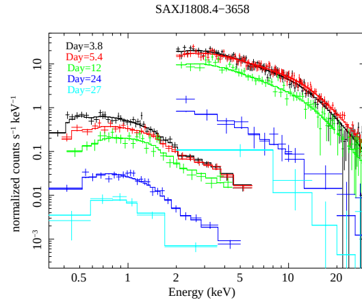
Fig. 19 Simulated combined SXI and XGIS spectra of SAX J1808.4-3658 for the 5 epochs shown in Fig. 18 adopting an absorbed power law with parameters as derived from Swift/XRT spectra. Exposure times were 2 ks for the first three epochs for both SXI and XGIS, while for the 4 th and 5 th epoch exposure times of 30 ks and 100 ks were assumed, respectively
