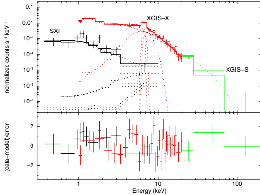
Fig. 10 A 25 ks exposure simulation of a nonmagnetic CV with 2-30 keV flux of 6 \times 10^{-12} \text{ erg cm}^{-2} \text{ s}^{-1} (see text for details). The count rates in the three detectors are 0.002 cts \text{s}^{-1} (0.3-6 keV), 0.074 cts \text{s}^{-1} (2-30 keV) and 0.0005 cts \text{s}^{-1} (30-150 keV).
