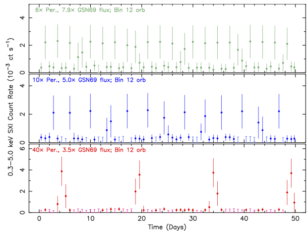
Fig. 27 A sample of simulated QPE light curves, based on the waveform observed in GSN 69 [255], and with binning every 12 satellite orbits. These light curves were produced by multiplying both the waveform and recurrence time observed in GSN 69 by factors of 6, 10, and 40 (top, middle, and bottom panels, respectively), and simulating peak 0.3–5 keV fluxes that are factors of 7.9, 5.0, and 3.5 times that observed in GSN 69. THESEUS SXI will be most sensitive to QPEs with periods of order tens of hours or longer, and fluxes a factor of at least a few times higher than that of GSN 69.
