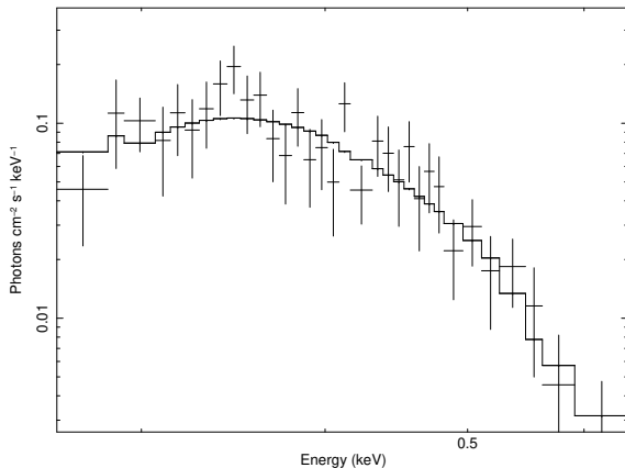
Fig. 31 Simulation of a typical, soft TDE ( kT=50 eV, N_H=1\times10^{21} cm ^{-2} ) observed for 20 ks with the SXI with a flux of \sim1\times10^{-11} erg cm ^{-2} s ^{-1} .
