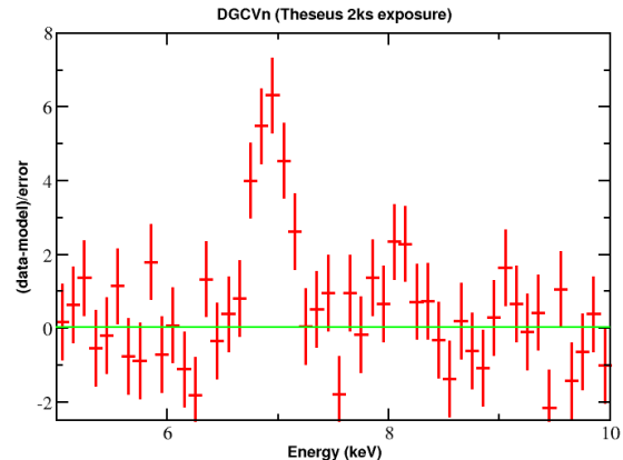
Fig. 7 Simulated residuals of a 2 ks XGIS-X spectrum showing Fe lines from the 280 MK optically thin thermal emission model fit to the Swift DG CVn super-flare [26] when fitted with a non-thermal bremsstrahlung model which fits the Swift data equally well. THESEUS is easily able to distinguish these models, constraining the plasma evolution on short timescales. The normalization of the model was chosen so that the fluxes in the 0.3-10 keV and 14-100 keV energy ranges are \sim 4 \times 10^{-9} \text{ erg cm}^{-2} \text{ s}^{-1} (i.e. similar to the fluxes of the first super-flare of DG CVn during 2014).
