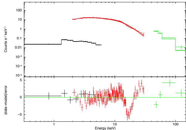
Fig. 16 Simulation of a SFXT spectrum in outburst (exposure time of 10 ks, SXI in black, XGIS-X in red, XGIS-S in green). The assumed model is an absorbed cutoff power law continuum modified by a cyclotron line at 17 keV, fitted by an absorbed cutoff power law with no line.
