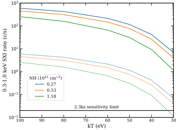
Fig. 11 Predicted SXI count rates from the as-yet undiscovered classical nova shock breakout derived from the model of Kato et al. [91]. The upper and lower sets of curves correspond to distances of 1 and 10 kpc, the typical Galactic range. The colours refer to differing absorbing column densities, corresponding to 25%, median and 75% of the cumulative distribution of Galactic HI values. The SXI detection limit for the standard unbroken observation length in the dynamic pointing scheme is shown. The peak temperature of the shock breakout is a measure of the mass of the WD, the range displayed covers the mass range of 1.3 - 0.6 M_{\odot} .
