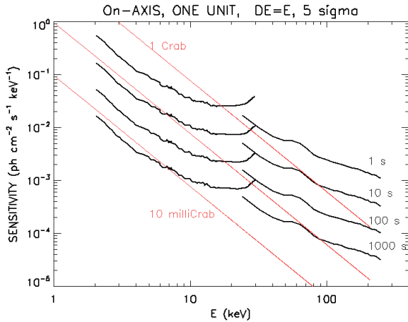
Fig. 3 XGIS imaging sensitivity ( 5\sigma c.l., \Delta E/E=1 ) for different exposure times. The curves refer to a single unit and sources in the fully coded field of view ( \sim 10 \times 10 \text{ deg}^2 ). One Crab corresponds to 3 \times 10^{-8} \text{ erg cm}^{-2} \text{ s}^{-1} in the 2-30 keV range and to 1.6 \times 10^{-8} \text{ erg cm}^{-2} \text{ s}^{-1} in the 30-150 keV range.
