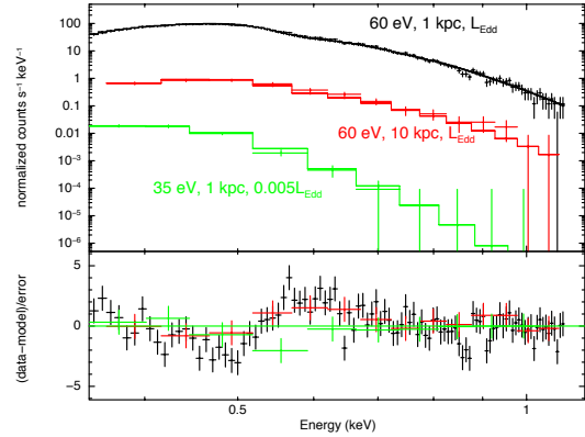
Fig. 12 A simulation of soft X-ray component spectrum of a nova for the SXI instrument using a 60 eV blackbody model with N_H = 2 \times 10^{21} \text{ cm}^{-2} . The black curve assumes a 60 eV blackbody emission with Eddington luminosity at d=1 \text{ kpc} , giving 21.1 \text{ cts s}^{-1} in the SXI, whereas the red curve is the same blackbody emission for d=10 \text{ kpc} simulated for the constant bolometric luminosity phase (2.5 ks, predicted rate 0.22 \text{ cts s}^{-1} ). The green curve represents a 0.005 L_{\text{Edd}} of a 35 eV cooling WD after X-ray turn-off with an exposure of 150ks and d=1 \text{ kpc} .
