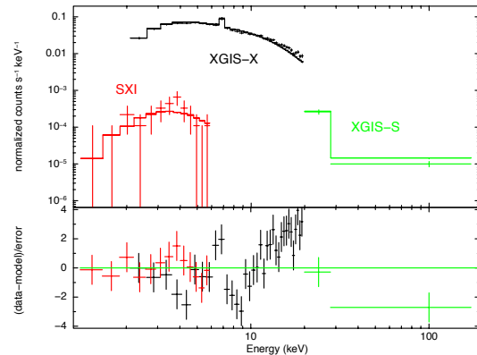
Fig. 9 A simulation of a 25 ks exposure of a MCV with THESEUS. The spectrum was simulated with a multi-temperature plasma emission model (with T_{\text{max}}=45 keV) and a Compton reflection component. An average intrinsic N_H of 5 \times 10^{22} \text{cm}^{-2} is assumed. The count rates are 0.0013 \text{cts s}^{-1} (0.3–6 keV), 0.66 \text{cts s}^{-1} (2–30 keV) and 0.0033 \text{cts s}^{-1} (30–150 keV). The bottom panel shows the residuals obtained when the reflection component is not included in the fit.
