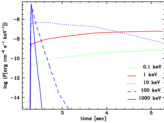
Fig. 33 Expected flux as a function of time for a Type Ia SN at 10 Mpc for the thermonuclear shock break out with a H/He/C mixed layer (peak luminosity = 5 \times 10^{48} erg s ^{-1} ), which can be detected with XGIS over 1 to 10 s [363,370,374].
