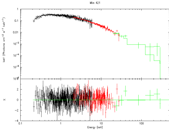
Fig. 29 Simulated SXI and XGIS spectra of Mkn421 (35 ks exposure, corresponding to 1 day of observation). An emission state similar to the one observed in April 2013 by INTEGRAL has been taken as a reference (i.e. the spectrum in the considered energy range is described by a logarithmic parabola with an energy cutoff at 10 keV (see [321])).
