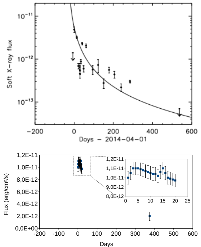
Fig. 30 Top: The lightcurve of XMM SL1J0740-85 observed with the XMM-Newton slew survey in the 0.2-2 keV band (reproduced with permission from [354]). Bottom : Simulation of a TDE lightcurve similar to XMM SL1J0740-85 as seen with the SXI. Details such as flares can be discerned, and the decay rate can easily be determined. Further dedicated pointed observations could also be taken to refine the long term lightcurve.
