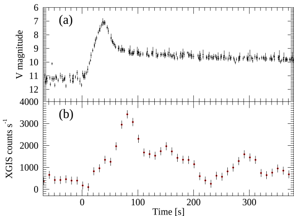
Fig. 8 a) Observed light curve of the optical emission of the initial part of the DG CVn super-flare [25]. b) Simulated XGIS light curve in the 2-30 keV energy range.
