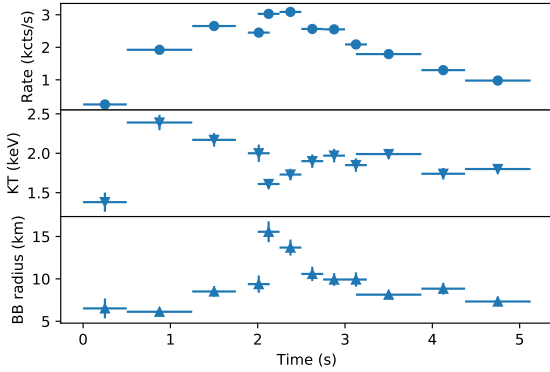
Fig. 21 Simulated on-axis XGIS light curve (upper panel) and spectral parameter evolution for a PRE burst (blackbody temperature in keV and black-body radius for an assumed 5 kpc distance in the middle and lower panels, respectively). Reference for this particular PRE burst template in [158].
