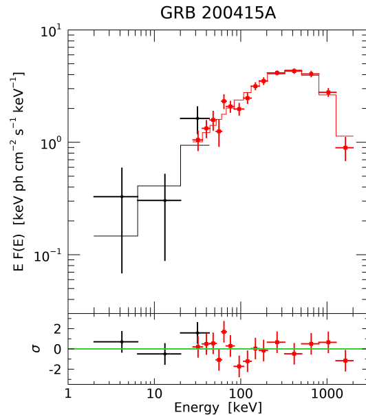
Fig. 23 XGIS-X (black) and XGIS-S (red) simulated spectra of the short GRB 200415A, possibly due to a magnetar located in the Sculptor galaxy (NGC 253).
