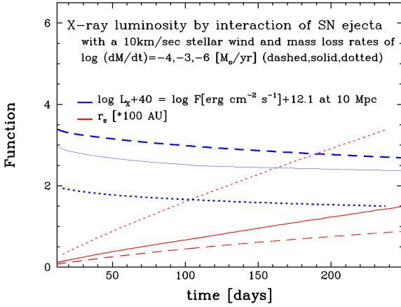
Fig. 34 Expected flux as a function of time for a Type Ia SN at 10 Mpc due to the interaction within the Roche-lobe with a mass-outflow 10^{-3} \dots 10^{-6} M_{\odot} , which may be within reach of SXI for integration times of 1 to 10 ks [363,370,374]. The onset of the interaction provides a direct measure of the size of the cavity and wind-properties of the progenitor.
