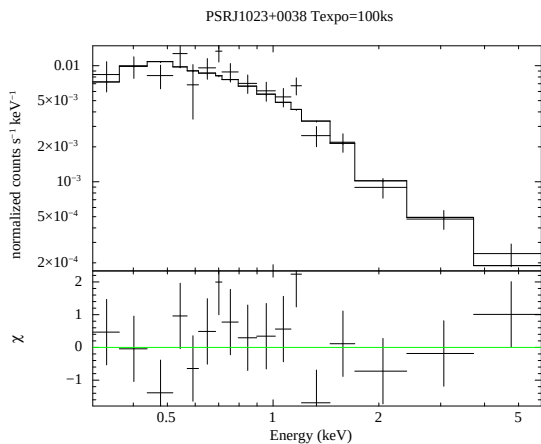
Fig. 20 Simulated SXI spectrum for PSR J1023+0038 in its current subluminal LMXB state adopting a 100 ks exposure and an absorbed power law with N_H = 3 \times 10^{20} \text{ cm}^{-2} and \Gamma=1.7 .
