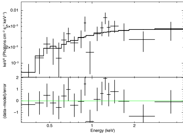
Fig. 25 THESEUS-SXI simulation of a nearby HLX in the low/hard state for an exposure time of 30 ks based on the observational properties of ESO 243–49 HLX–1 from [221].
