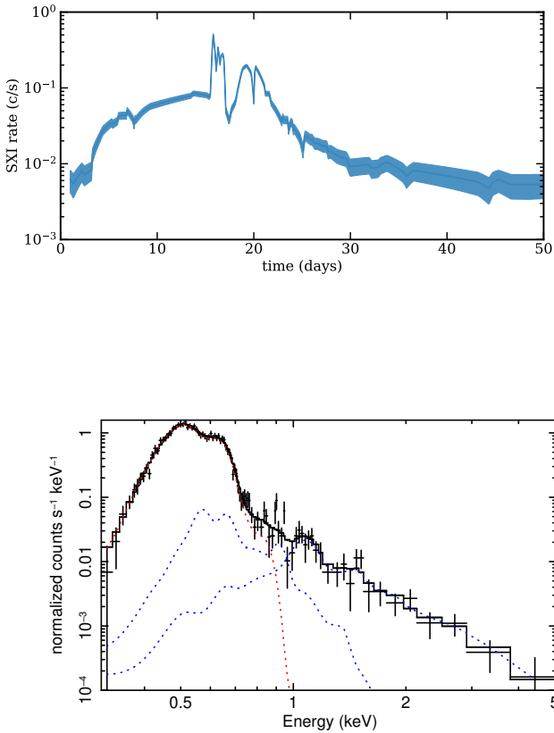
Fig. 13 (a) The top figure shows the predicted SXI count rates that would have been seen from the recurrent nova V3890 Sgr, derived from Swift/XRT observations [95]. The shaded region denotes the 1\text{-}\sigma Poisson error range expected for an exposure time of 2.3 ks, typical for THESEUS visits. (b) The bottom figure shows the predicted SXI spectrum on day 20 of the outburst, as simulated for an exposure of 20 ks (i.e. multiple visits combined) to reveal the hard component. The supersoft source emission dominates the SXI count rate, with the shocked ejecta contributing only 10% of the emission on day 20.
