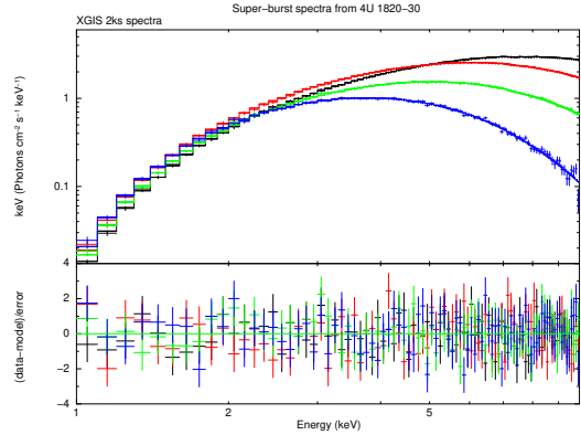
Fig. 22 Simulated XGIS time-resolved spectra of the cooling evolution of a superburst event. Each spectrum has an assumed exposure of 2 ks.
