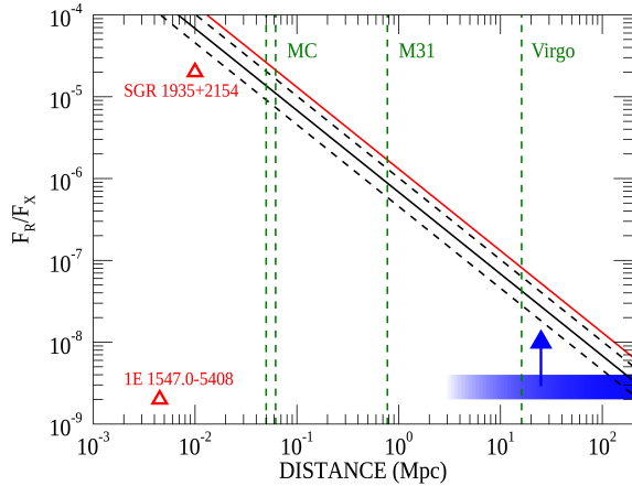
Fig. 35 Maximum distance for detection of a burst from a FRB for SXI (black) and XGIS (red) as a function of the ratio between radio and X-ray fluence F_R/F_X (see text for details). For these estimates we scaled the properties of the 2020 April 28 burst, using the Hard X-ray Modulation Telescope X-ray spectrum [403] for the SXI estimates, and the INTEGRAL spectrum [402] for the XGIS ones. For the SXI we have required a minimum fluence of 5 counts, which constitutes a significant detection in the observed duration ( \sim 0.5 s) of these short events. The dashed lines indicate the range of uncertainty due to the unknown absorption (they refer to N_H = 10^{20} and 10^{22} \text{cm}^{-2} ). The red triangles indicate the only values of F_R/F_X measured to date from two Galactic magnetars, while the blue region indicates typical lower limits inferred from the non-detection of high energy emission from extragalactic FRB. The green dashed lines indicate the distances of the Magellanic Clouds, the Andromeda galaxy and the Virgo cluster.
