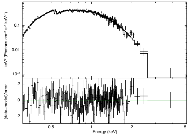
Fig. 26 THESEUS-SXI simulation of a nearby HLX in the high/soft state for an exposure time of 30 ks based on the observational properties of ESO 243–49 HLX–1 from [221].
