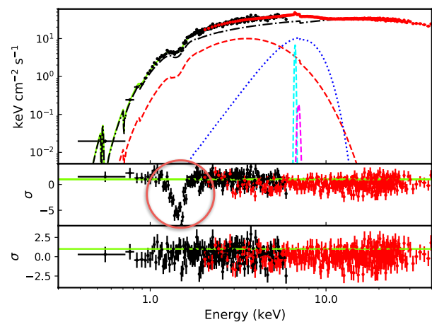
Fig. 17 THESEUS simulation of a proton cyclotron absorption line in the continuum spectrum of the transient PULX Swift J0243.6+6124 for an X-ray luminosity of 10^{39} erg s ^{-1} using an absorbed black body and cut-off power-law plus some additional iron lines and its edge, based on the spectrum of the source during the 2017-2018 strong outburst [127]. SXI in black, XGIS in red. The simulated proton cyclotron line corresponds to a magnetic field of 3 \times 10^{14} G. In the middle panel, the line at \sim 1.45 keV is clearly identified. The residuals after a Gaussian absorption line is added are shown in the bottom panel.
