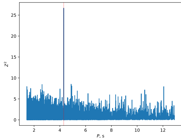
Fig. 14 Simulated periodogram for 10 ks THESEUS/SXI observation (typical daily exposure) for a representative transient X-ray pulsar with bolometric flux of 10^{-9} \text{ erg cm}^{-2} \text{ s}^{-1} , spin period of 4.3 s and pulsed fraction of 20% (excluding background).
