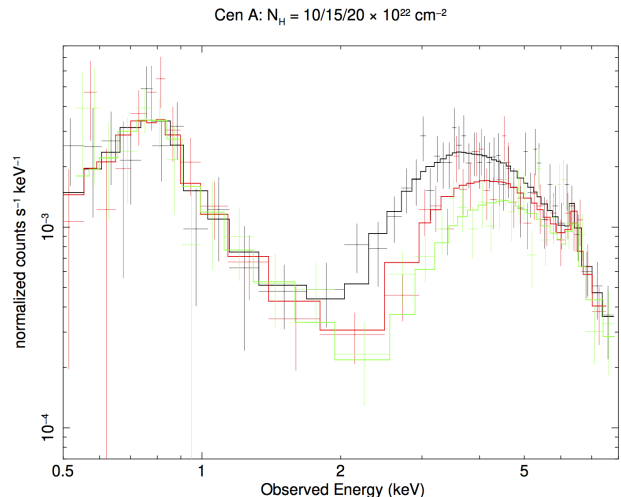
Fig. 28 Simulated SXI spectra of Cen A. THESEUS SXI can track fluctuations in line-of-sight column density N_H as density variations in its clumpy torus drift across the line of sight. Shown here are spectra corresponding to columns of 10, 15, and 20 \times 10^{22} \text{ cm}^{-2} , (black, red, and green, respectively, based on variations observed by [287]), each 70 ks accumulated exposure.
