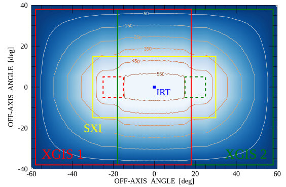
Fig. 2 Fields of view of the THESEUS instruments. The red (left) and green (right) squares indicate the partially coded FoV ( 77 \times 77 \text{ deg}^2 , solid lines) and fully coded FoV ( 11 \times 11 \text{ deg}^2 , dashed lines) of the two XGIS units. The yellow rectangle is the SXI FoV ( 61 \times 31 \text{ deg}^2 ). The blue square indicates the pointing direction of the IRT. The contour lines indicate the effective area at 10 keV provided by the sum of the two XGIS units, assuming a 50% open fraction for the coded masks.
