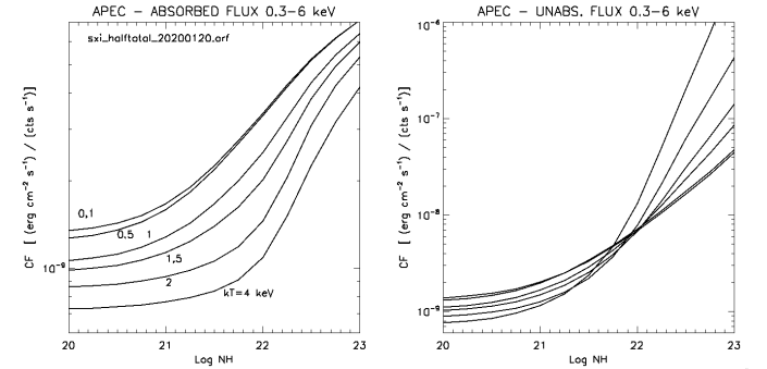
Fig. 38 SXI counts to flux conversion rates for a thermal plasma spectrum (APEC in XSPEC) as a function of absorption. The lines refer to different temperatures. The left figure refers to absorbed fluxes and the right one to fluxes corrected for the absorption.
