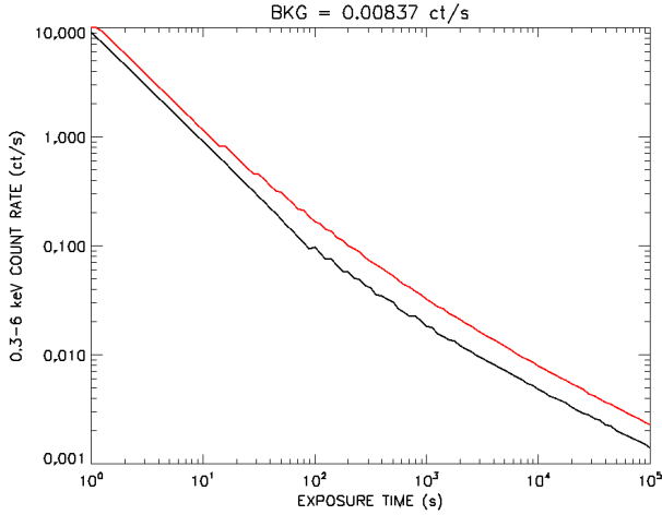
Fig. 36 SXI sensitivity as a function of exposure time. The lower curve (black) gives the count rate corresponding to a 95% probability to exceed a threshold of 3\sigma ( P_1=1.35 \times 10^{-3} ), while the upper curve (red) gives the count rate corresponding to a 99% probability to exceed a threshold of 5\sigma ( P_1=3 \times 10^{-7} ). The assumed background rate of 8.371 \times 10^{-3} cts s^{-1} is appropriate for a source extraction region of 675 arcmin ^2 .
