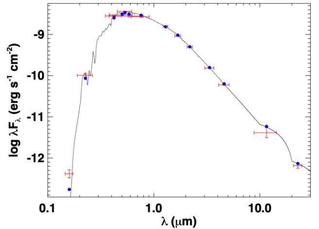
Figure 1. SED of TOI-282. Red symbols represent the observed photometric measurements, where the horizontal bars represent the effective width of the passband. Blue symbols are the model fluxes from the best-fitting Kurucz atmosphere model (black).
