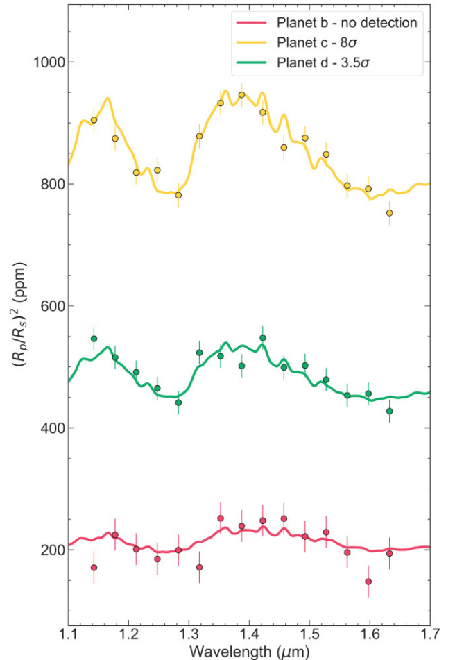
Figure 14. Model transmission spectra of HD 28109 b, c, and d with simulated HST observations. Each point corresponds to a single transit depth with no offset; the curves represent the simulated transmission spectra.
