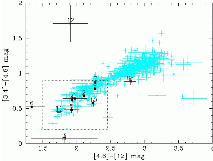
Fig. 5. [4.6] - [12] / [3.4] - [4.6] MIR colour-colour plot reporting the positions of gamma-ray emitting blazars (in cyan) associated with WISE sources forming the blazar strip (see Massaro et al. 2013a for more details), together with the BL Lac objects identified in this paper. Filled and unfilled squares depict the proposed associations flagged with L or P in the last column of Table 3, respectively.
