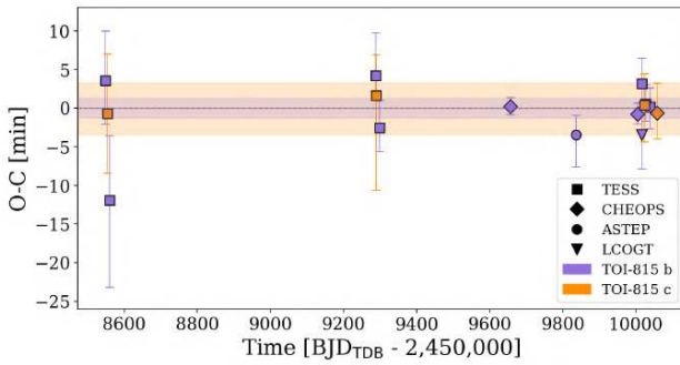
Fig. 14. Transit timings for each transit of TOI-815b (purple) and TOI-815c (orange) measured from the TESS and CHEOPS light curves. The purple and orange regions represent the 1\sigma uncertainties of the inner and outer planet ephemeris reported in Table E.1.
