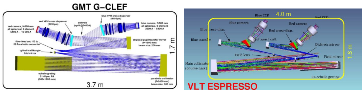
Figure 24 Layouts of the G-CLEF (left panel) and ESPRESSO spectrometers
