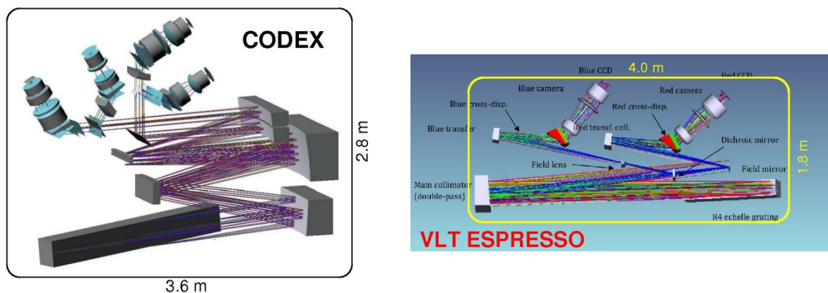
Figure 25 Layouts of the CODEX (left panel) and ESPRESSO spectrometers
