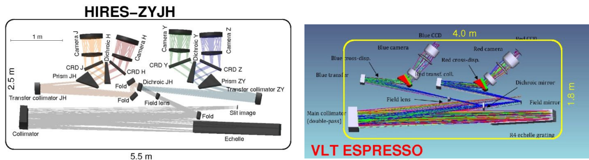
Figure 26 Layouts of the HIRES (left panel) and ESPRESSO spectrometers
