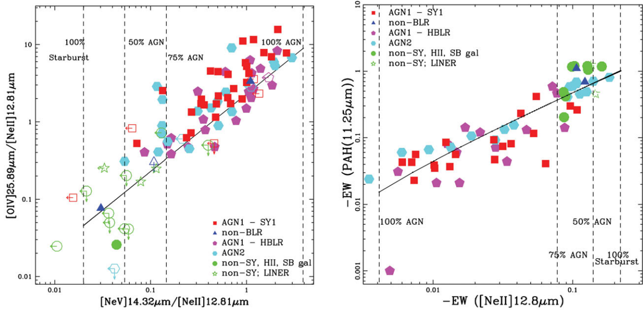
Figure 3. Left panel: [Ne\text{V}]14.3\mu\text{m}/[Ne\text{II}]12.8\mu\text{m} line ratio versus [O\text{IV}]25.9\mu\text{m}/[Ne\text{II}]12.8\mu\text{m} line ratio. Both axes correlate with the strength of the AGN. The black line shows the behaviour of the analytical model (Tommasin et al. 2010). Right panel: [Ne\text{II}]12.8\mu\text{m} equivalent width versus PAH 11.25\mu\text{m} equivalent width. Both quantities in this plot correlate with the strength of the star-formation component in each galaxy. The black line shows the behaviour of the analytical model (Tommasin et al. 2010).
