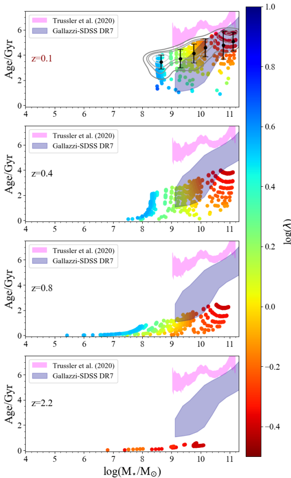
Fig. 12. As in Fig. 6, but computed assuming a constant SFE fixed at the value of 1 \text{ Gyr}^{-1} .
