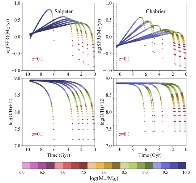
Fig. A.6. Evolution of star formation rate ( upper panels ) and oxygen abundance ( lower panels ) as a function of time for the galaxies with infall mass M_{\text{inf}} = 10^{10.5} M_{\odot} that lie on the MZR of Kewley & Ellison (2008) and on the MSR as derived by Peng et al. (2010) , computed assuming a Salpeter (1955) IMF ( left panels ) and a Chabrier (2003) IMF ( right panels ). The color-coding stands for the stellar mass.
