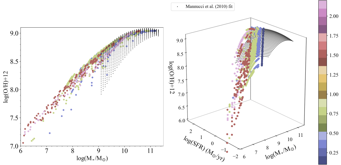
Fig. 11. Two projections of the FMR of Mannucci et al. (2010) compared with the properties of the model galaxies as in Fig. 10, colour-coded as a function of their redshift z .
