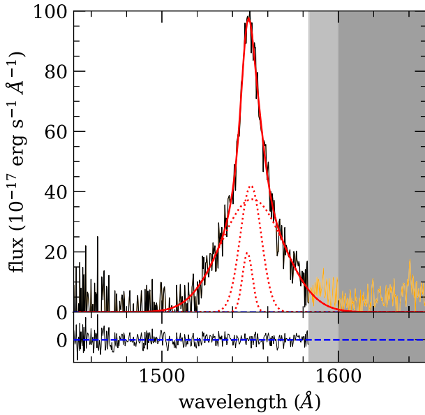
Figure 1. Example of the fitting procedure (GB6J162030+490149). The top panel represents the rest-frame continuum-subtracted spectrum. The mask applied is represented with the grey shaded area and in orange is shown the excluded part of the spectrum. The best-fitting model for the C IV line is represented with the solid red line, while the single Gaussian components are depicted with the dotted red line. The bottom panel shows the residuals.
