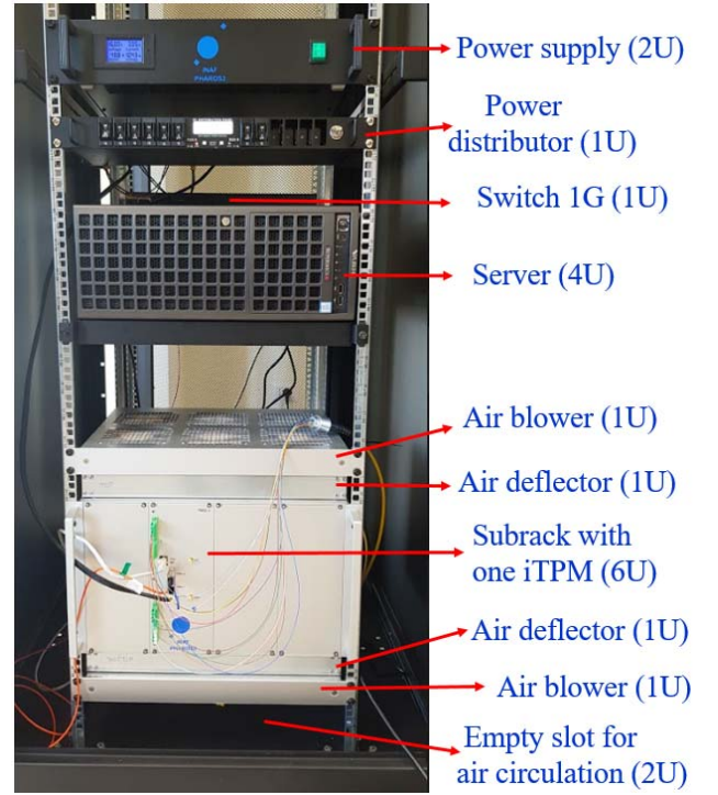
Fig. 19. Digital backend cabinet showing a subrack with one iTPM and air blower for air circulation (bottom), the server, the power supply, the power distributor and the network switch (top).
