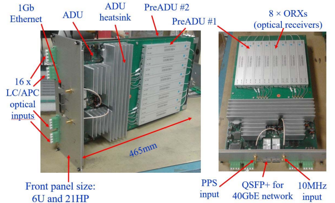
Fig. 18. iTPM digital backend consisting of the Analog Digital Unit (ADU) and of two preADU boards. Each preADU boards contains eight fiber-optics receivers (ORXs).
