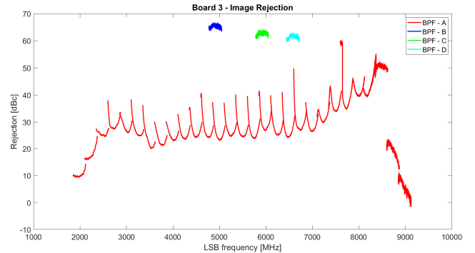
Fig. 13. Image sideband rejection measured for one of the channels (ch.1) of WS RF/IF Board #3 across the four different band pass filters. The \approx 2-9 GHz LSB signal frequency for BPF-A was covered by 29 different LO frequency settings (red curves). Measured image rejection across BPF-B, C and D are shown by curves in dark blue, green and light blue, respectively. For each given LO frequency, the rejection values refer to the 375-650 MHz IF frequency band (275 MHz bandwidth).
