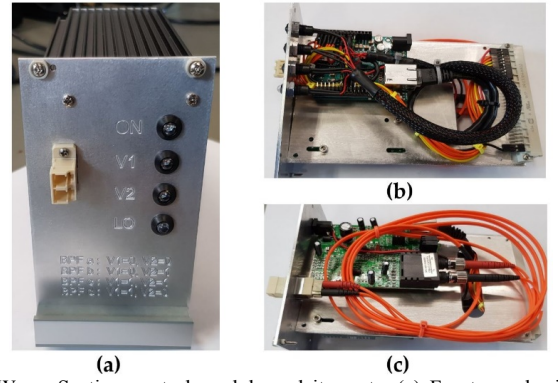
Fig. 8. Warm Section control module and its parts. (a) Front panel with TX/RX multimode fiber connector pair and LEDs. (b) Microcontroller by Arduino Leonardo ETH. (c) Optical fiber to Ethernet media-converter (Digitus DN-82010).
