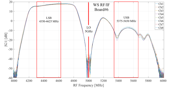
Fig. 10. VNA measured transmissions of the eight channels of one of the WS RF/IF boards by selecting filter BPF-A and LO frequency 5 GHz.
