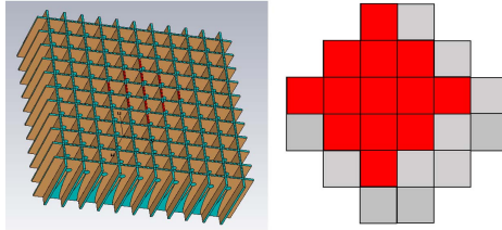
Fig. 4. Sub-array of 13 Vivaldi elements of the 24 active antennas connected to one analogue beamformer of the PHAROS PAF. Excited stripline antenna ports of Beam 1 (in red) and subset of the 24 active antennas (right panel).
