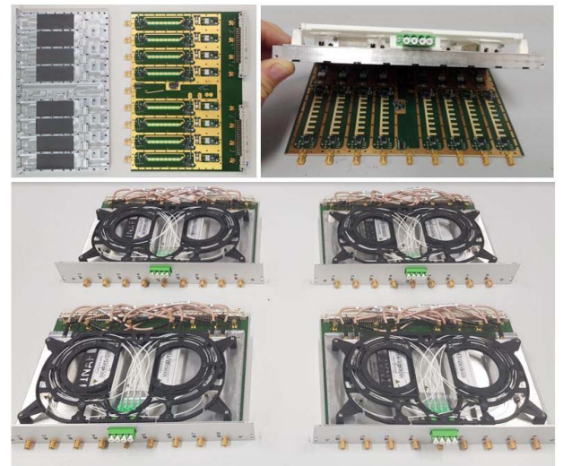
Fig. 6. Photos of the WS RF/IF module. Top left: mechanical housing (left) and fabricated PCB (right) before assembly. Microwave absorbers are glued in the pockets of the PCB mechanical housing. Top right: PCB board (first prototype version) and mechanical housing during assembly with optical transmitters. Bottom: Four WS RF/IF modules fully assembled, with OTXs.
