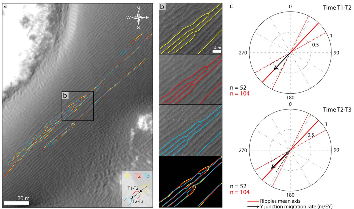
Figure 3. (a) Longitudinal migration of the LRs at T1–T3. (b) Zoom-in showing the longitudinal Y junction migration in the three frames. (c) Circular plot showing the comparison between the mean average Y junction migrations (in meter) and the mean bed form trend (circular standard deviation intervals are also shown) in the two study periods T1–T2 and T2–T3. Note that the Y junction migration direction is nearly longitudinal to the mean bed form trend and that the rate of migration is similar in the two analyzed intervals.
