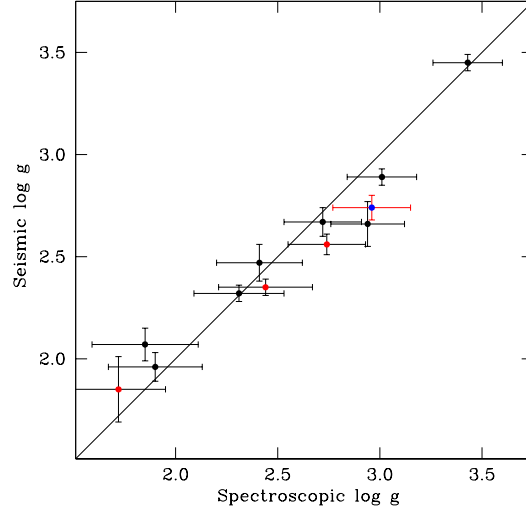
Fig. 2 Agreement between \log g values obtained from seismic and spectroscopic analyses. Red circles: red giants belonging to NGC 6633; blue circle: HD 170031; black circles: galactic red giants.
